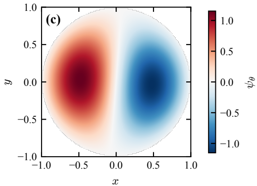
PINN 3, \epsilon = 14.682
