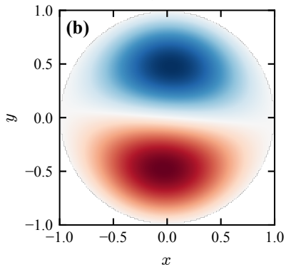
PINN 2, \epsilon = 14.682
