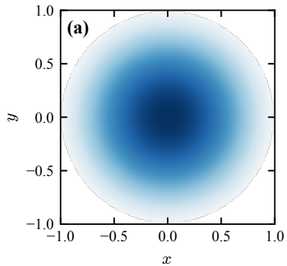
PINN 1, \epsilon = 5.783
