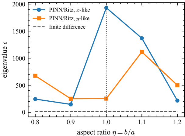
elliptic deformation splits the m = 1 doublet
