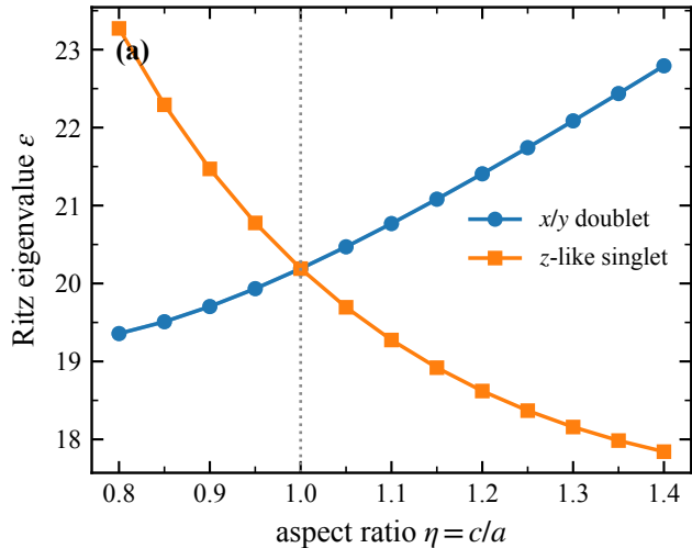
SO(3) \rightarrow SO(2) splitting
