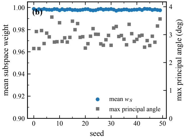
subspace recovery across seeds
