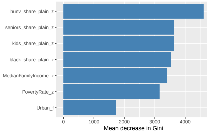
Figure 4: Random forest variable importance (mean decrease in Gini).
