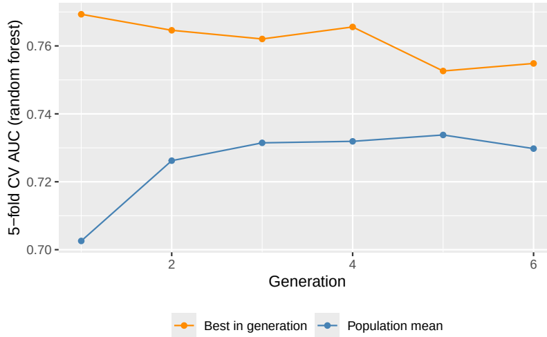
Figure 3: Genetic algorithm convergence: best and mean 5-fold CV AUC by generation.
