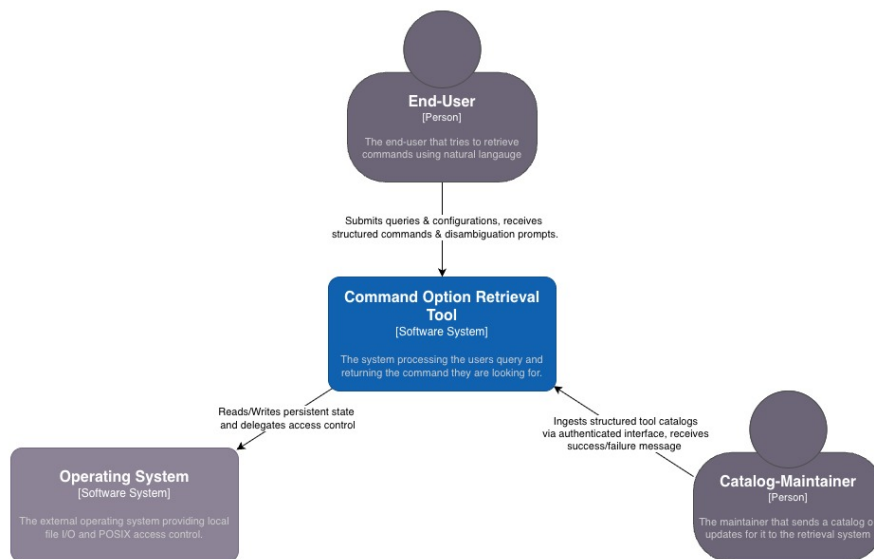
Abbildung 1: Level 1 System Context Model
