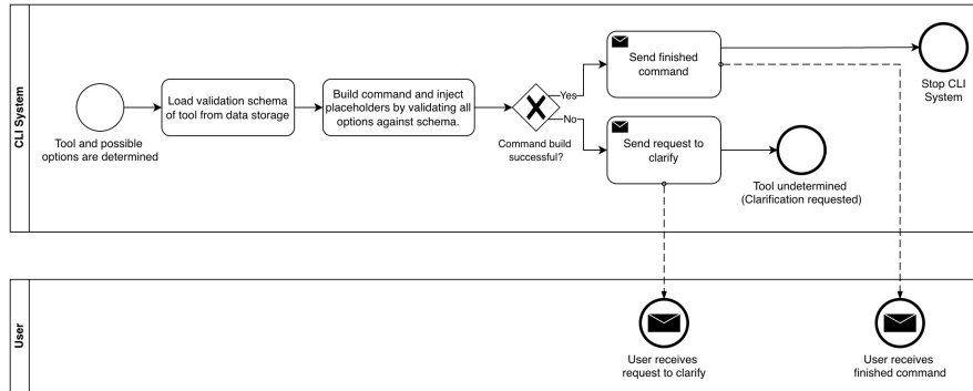
Abbildung 7: BPMN High-Level Systems Overview for Query Resolution
