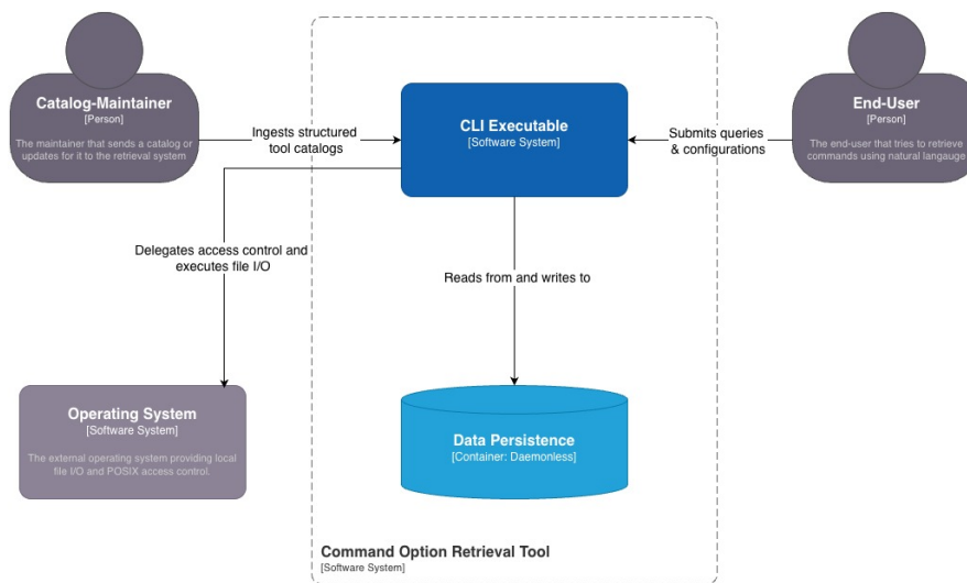
Abbildung 2: Level 2 Container Architecture
