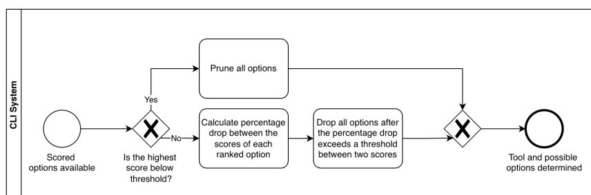
Abbildung 6: BPMN High-Level Systems Overview for Query Resolution
