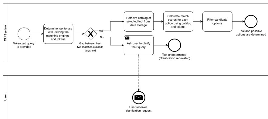
Abbildung 5: BPMN High-Level Systems Overview for Query Resolution
