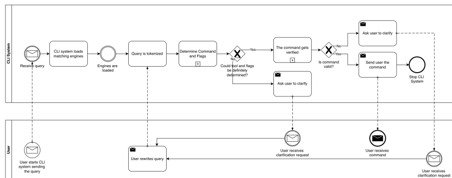
Abbildung 4: BPMN High-Level Systems Overview for Query Resolution
