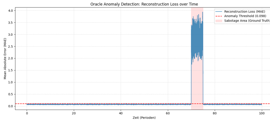
Figure 2: Oracle Anomaly Detection
