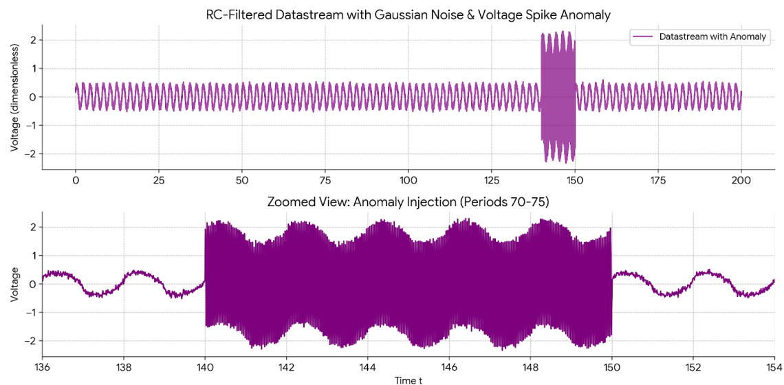
Figure 1: Sabotage Plot
