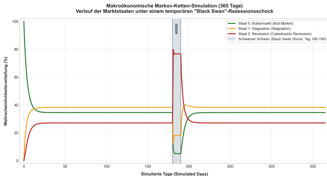
Figure 6: Markov Chain State Distribution
