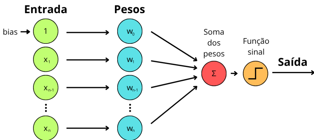
Figura 1 – Perceptron
