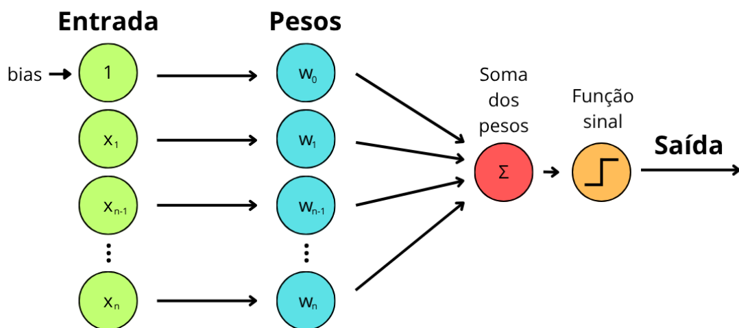
Figura 1 – Perceptron
