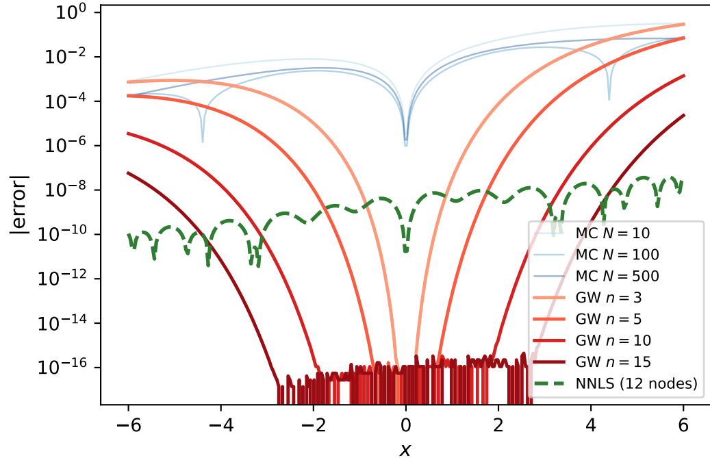
Absolute error vs exact \sigma(x)
