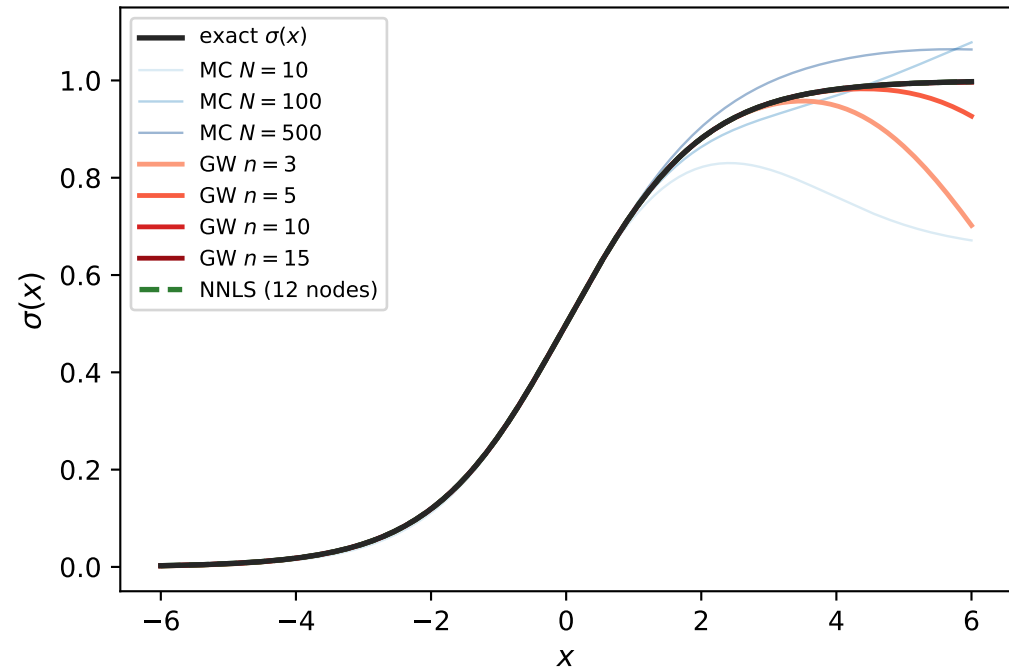
PG-sigmoid identity: MC vs quadrature
