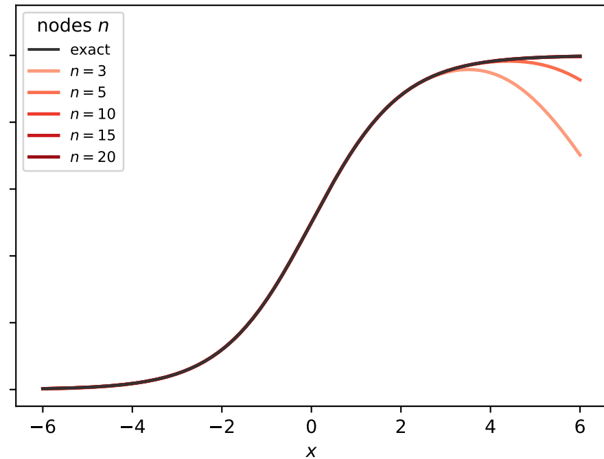
Gauss-PG quadrature
