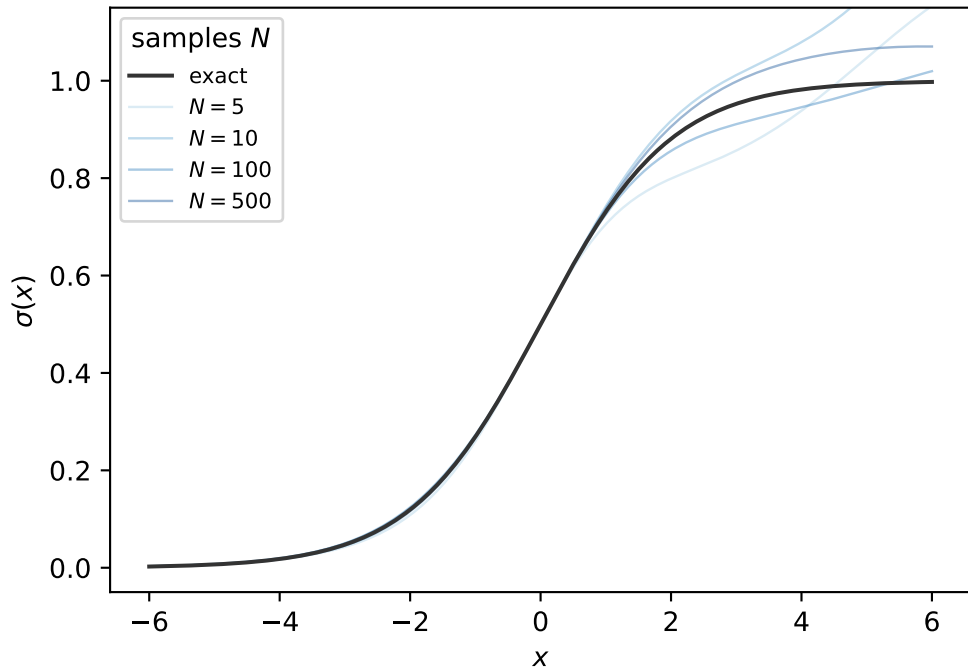
MC sampling
