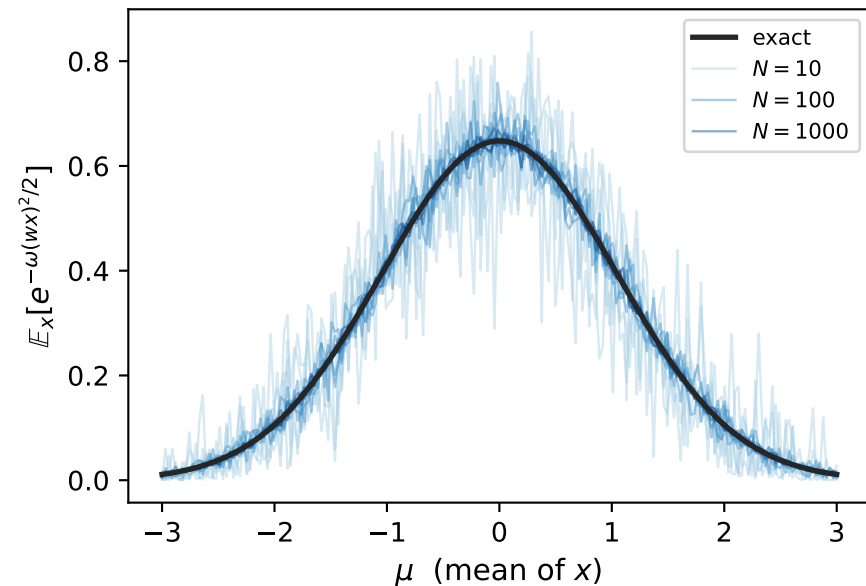
Direct MC over x
