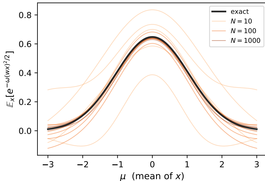
HS trick: MC over u , CF in closed form
