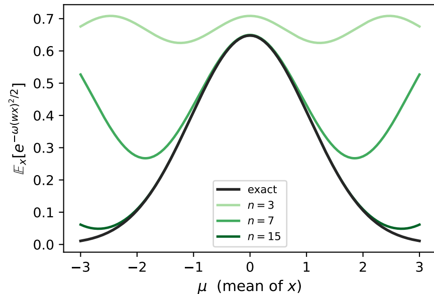
HS trick: Gauss-Hermite over u
