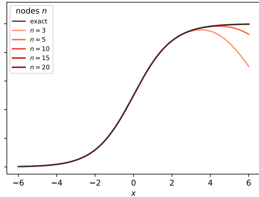
Gauss-PG quadrature
