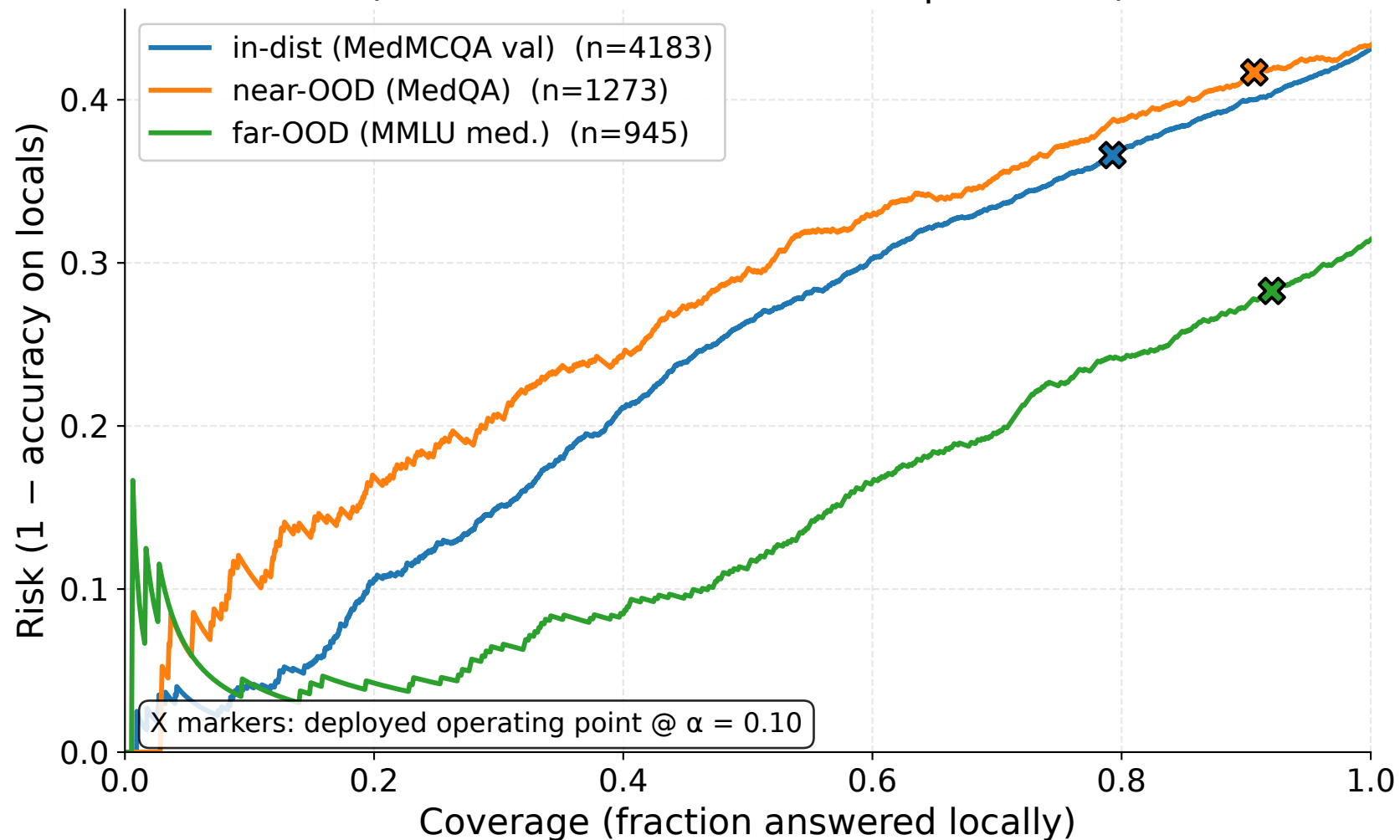
Risk-Coverage curves (lower-left = better selective prediction)
