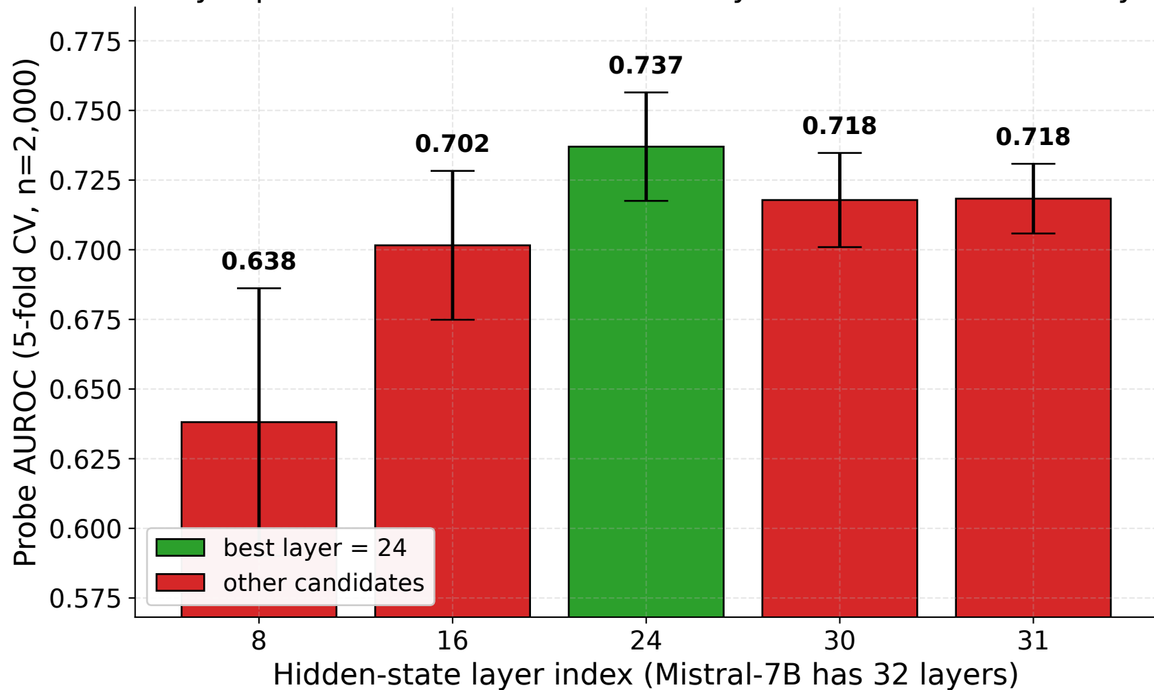
Per-layer probe AUROC — late-middle layers win over the final layers
