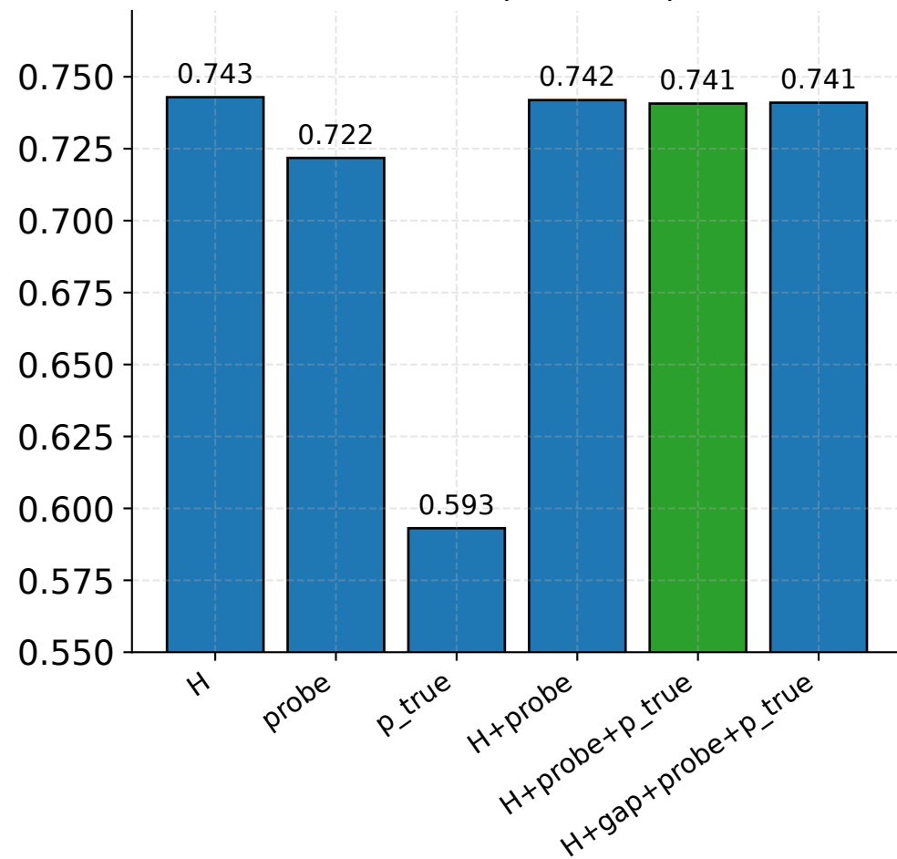
AUROC (↑ better)
