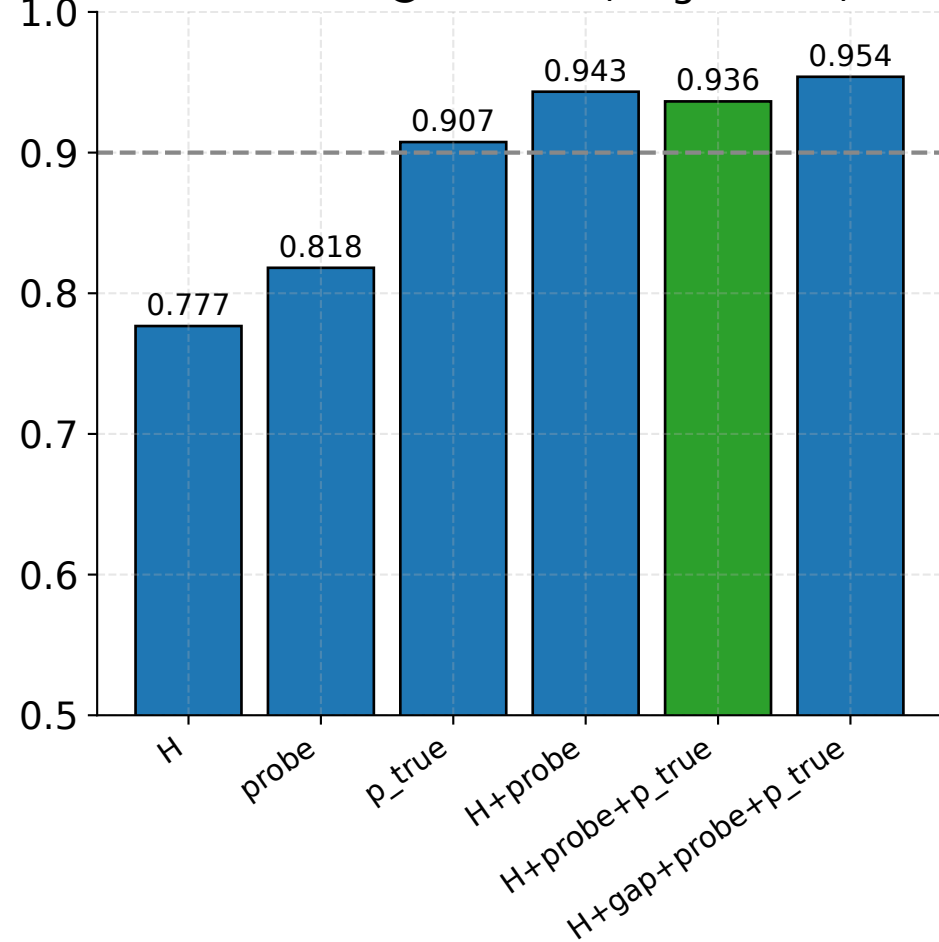
local rate @ \alpha=0.10 (target 0.90)
