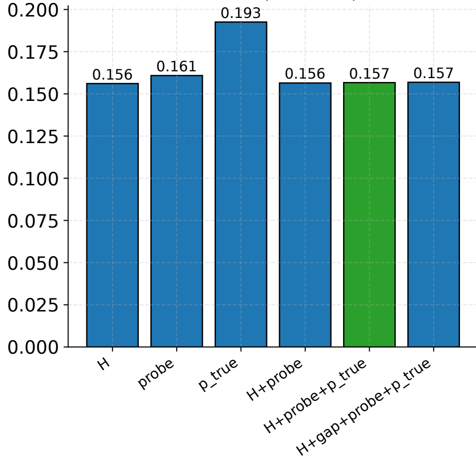
AUGRC (↓ better)
