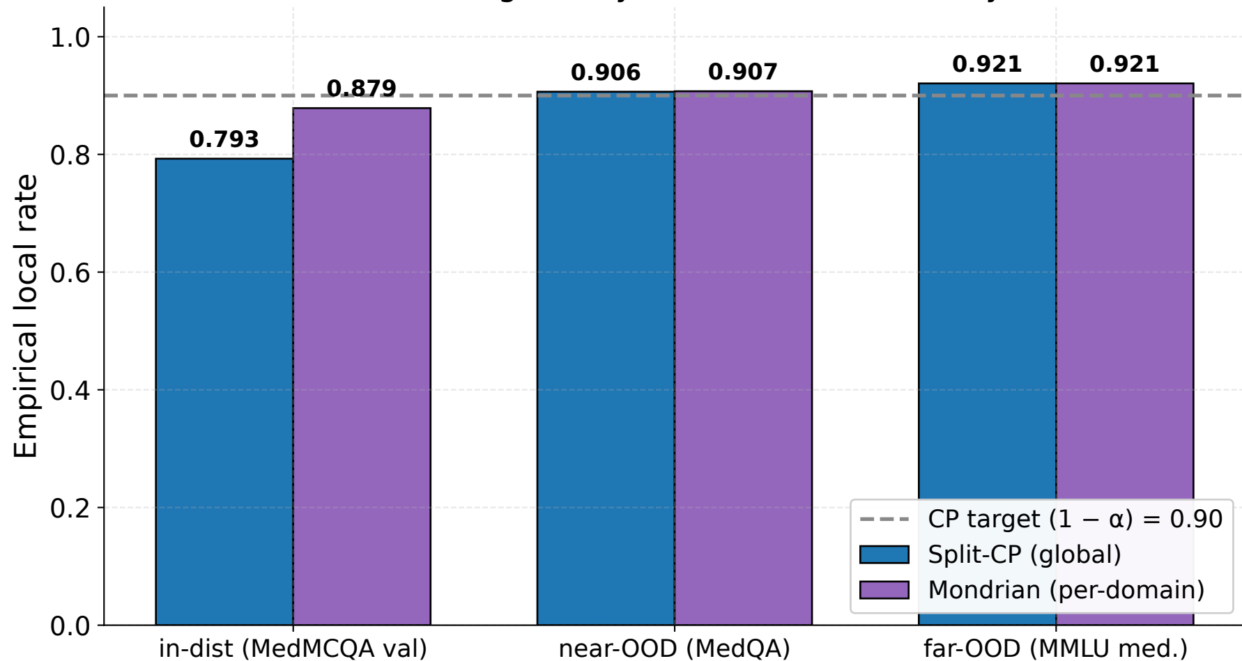
Split-CP vs Mondrian CP — per-domain stratification partially fixes the in-distribution exchangeability issue (but doesn't fully reach 0.90)
