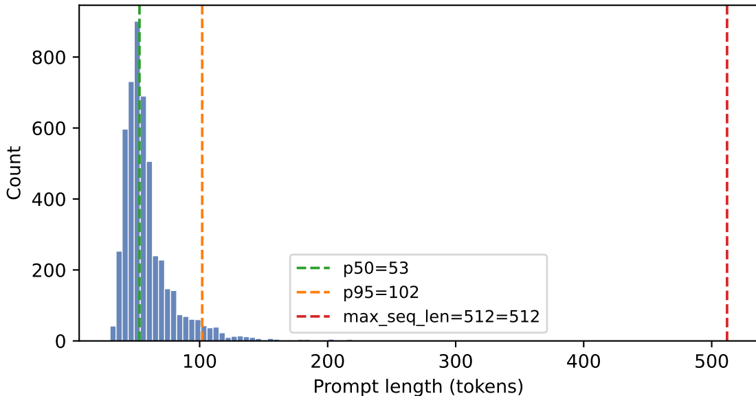
Full prompt length — MedMCQA (n=5,000 sample)
