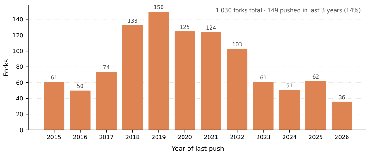
Figure 7: Last-push year distribution for the 1,030 enumerable Consul forks (snapshot 2026-05-12). Each bar counts forks whose most recent push falls in that year. Activity peaks in 2019 and declines; only 14% of forks have been touched since the start of 2024.
