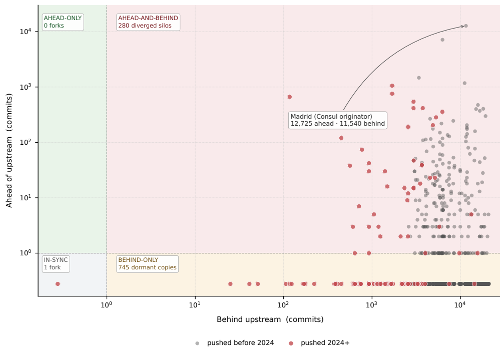
Figure 6: Consul forks plotted by commits ahead of upstream master against commits behind, on log scales (snapshot 2026-05-12). Each fork occupies one of four quadrants. The ahead-only region — where healthy contributor forks would live — is empty: no fork has added local commits while staying in sync with upstream. The mass sits in the behind-only region (745 dormant copies) and the ahead-and-behind region (280 diverged silos, including Madrid). Of 1,030 enumerated forks, 1,026 had upstream comparison data; the remaining four are excluded.
