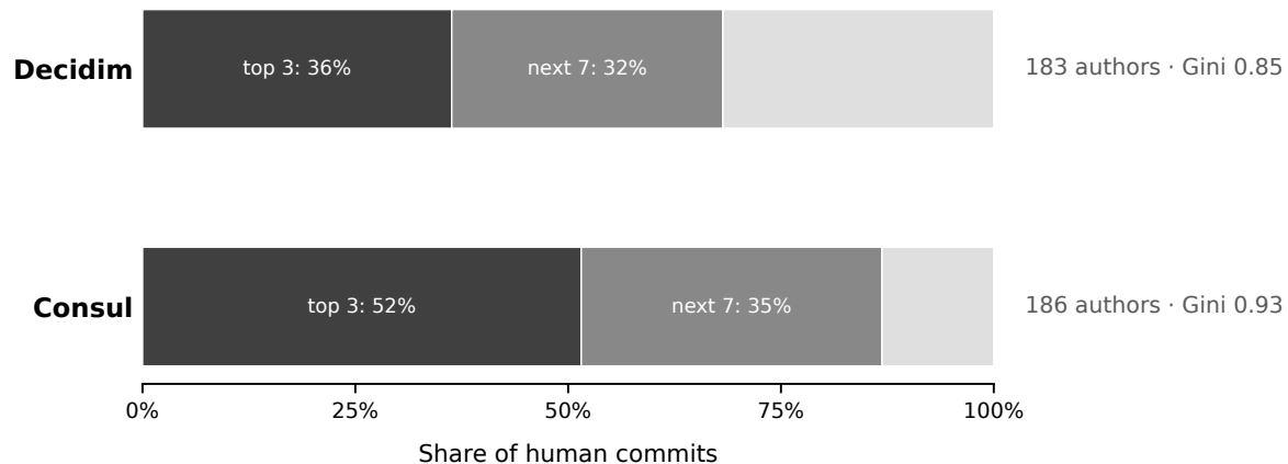
Figure 8: Share of human commits captured by the top three and top ten authors per repository. Decidim has a longer tail of unique contributors; Consul is more concentrated. Bot commits (Dependabot, Crowdin, etc.) are excluded.
