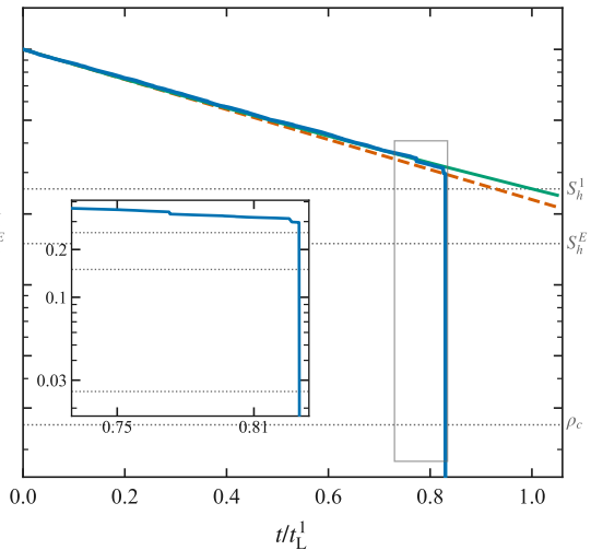
(b) Case II (brittle, C = 0.75 C^* )
