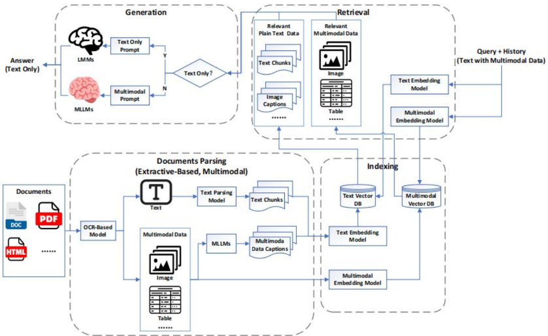
Fig. 2. The architecture of MRAG2.0 ( <Desc>2.png</Desc> ) retains multimodal data through document parsing and indexing, while introducing multimodal retrieval and MLLMs for answer generation, truly entering the multimodal era.
