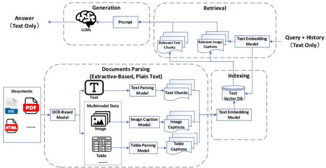
Fig. 1. The architecture of MRAG1.0 ( <Desc>1.png</Desc> ), often termed "pseudo-MRAG", closely resembles traditional RAG, consisting of three modules: Document Parsing and Indexing, Retrieval, and Generation. While the overall process remains largely unchanged, the key distinction lies in the Document Parsing stage. In this stage, specialized models are employed to convert diverse modal data into modality-specific captions. These captions are then stored alongside textual data for utilization in subsequent stages.
