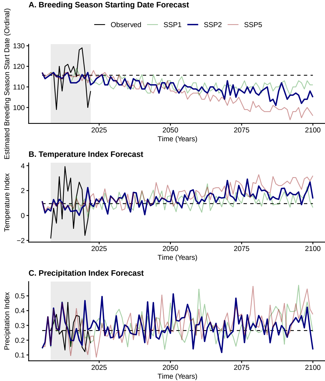
Figure B1: Time series of observed (black), and forecasted (coloured) indices, from 2005 to 2100. Panels A, B, and C display breeding season start date, temperature, and precipitation indices respectively. The grey shaded areas represent the BLISS study period (2008 to 2022), and the horizontal dashed lines indicate the average observed index values during this period. The climate scenario labelled ‘SSP2’ is emphasized for visual contrast.
