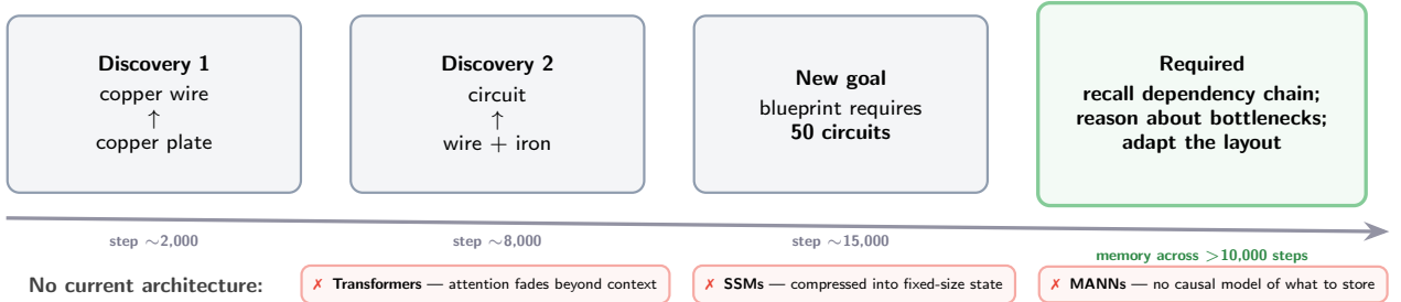
Figure 2: The capability gap FIND addresses. An agent discovers dependencies thousands of steps apart and must later recall and compose them under a new goal. This requires selective storage, content-addressable recall, and causal reasoning across >10,000 timesteps—beyond current architectures (bottom).
