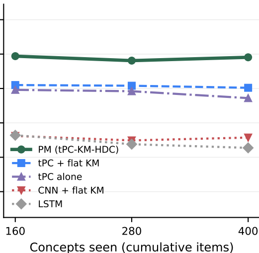
(B) Continual multi-class learning ( \sigma = 0.5 )
