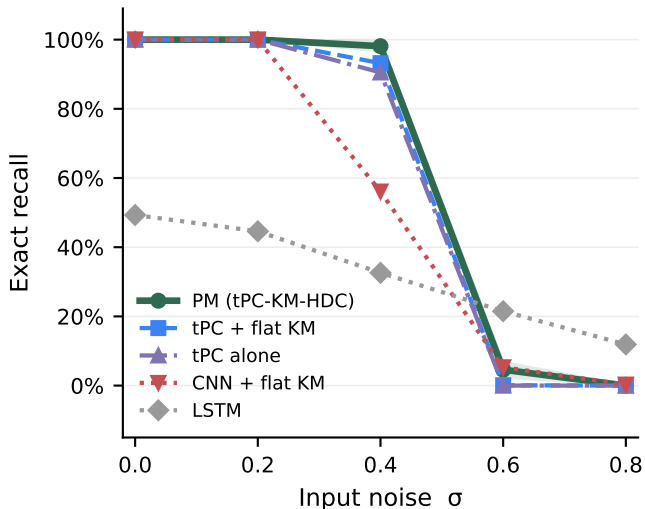
(A) Noise robustness (K = 100)
