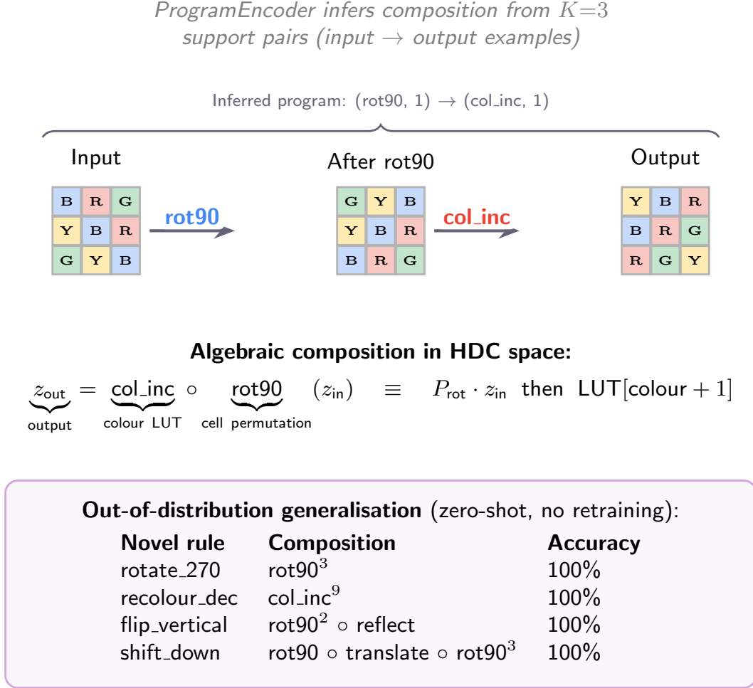
Figure 7: Compositional reasoning through algebraic operations in HDC space. A visual transformation (rotation + colour increment) is decomposed into composable primitives. The ProgramEncoder infers the composition from support examples. Algebraic composition guarantees out-of-distribution generalisation to novel rules without retraining (bottom table).
