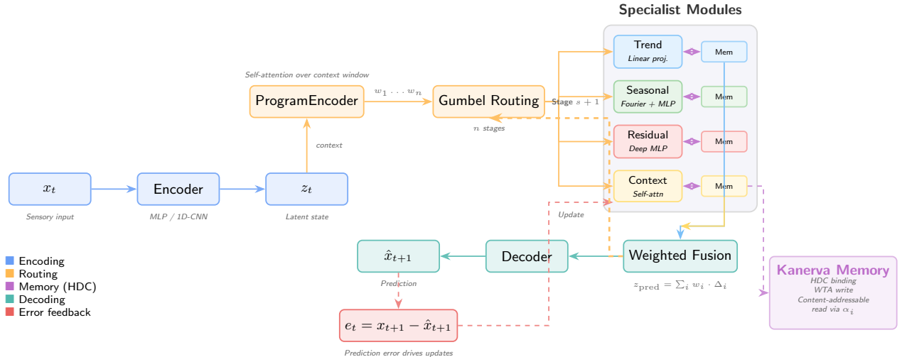
Figure 3: PAM architecture. Sensory input x_t is encoded into latent state z_t . A ProgramEncoder infers routing weights via self-attention over the context window. Gumbel-softmax routing selects among four specialist modules (Trend, Seasonal, Residual, Context), each with dedicated Kanerva memory using HDC binding for content-addressable read/write. The routing is applied iteratively over n stages. Module outputs are fused into a prediction \hat{x}_{t+1} ; prediction errors drive parameter updates. The module inventory is task-dependent (shown here for temporal forecasting).
