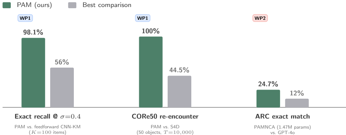
Figure 5: Headline preliminary results. PAM against the strongest comparison on each benchmark: noisy sequence recall at \sigma=0.4 (WP1 foundation), CORE50 re-encounter recognition after T=10,000 steps (WP1), and ARC program synthesis via test-time training (WP2).
