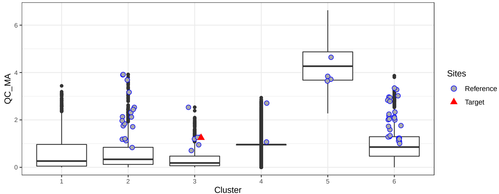
Mean annual flow (est.) (cfs) in the catchment by cluster
