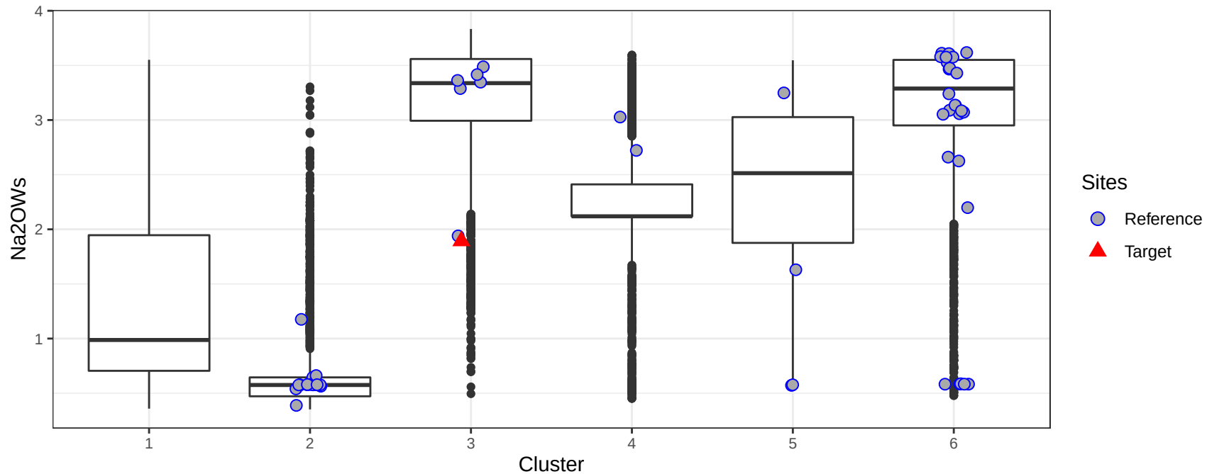
Surface Na 2 O content (%) in the watershed by cluster
