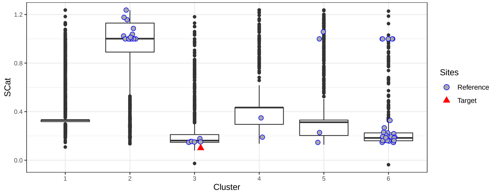
Surface S content (%) in the catchment by cluster
