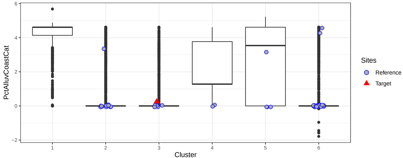
Alluvium and fine-textured coastal zone sediment (%) in the catchment by cluster
