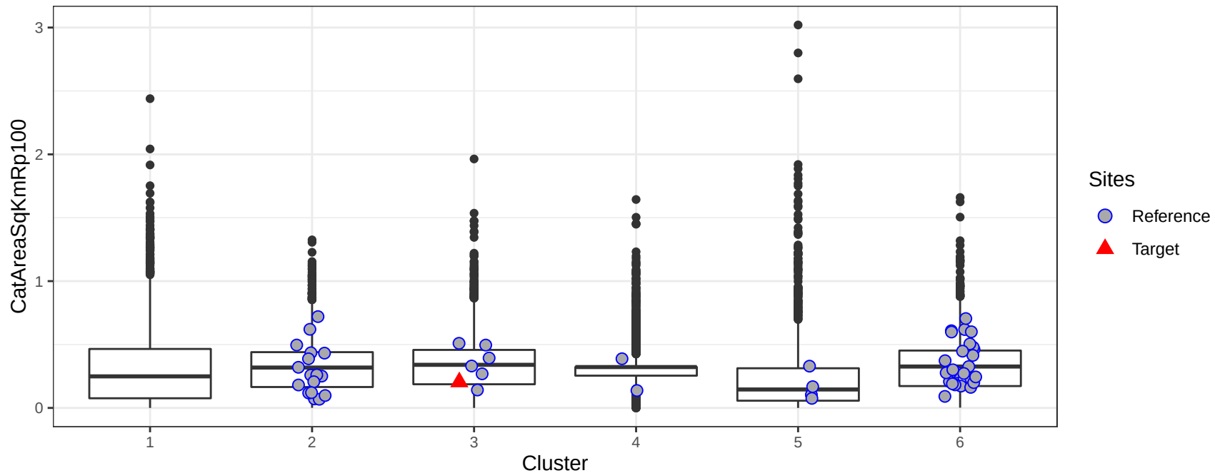
Area within the riparian buffer (sq. km.) in the catchment riparian by cluster
