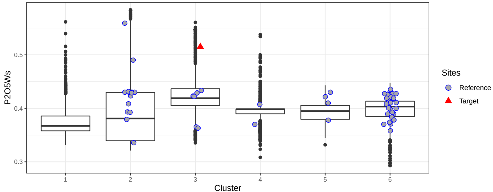
Surface P2O5 content (%) in the watershed by cluster
