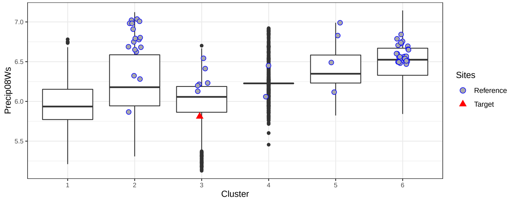
Mean precipitation in 2008 (mm) in the watershed by cluster
