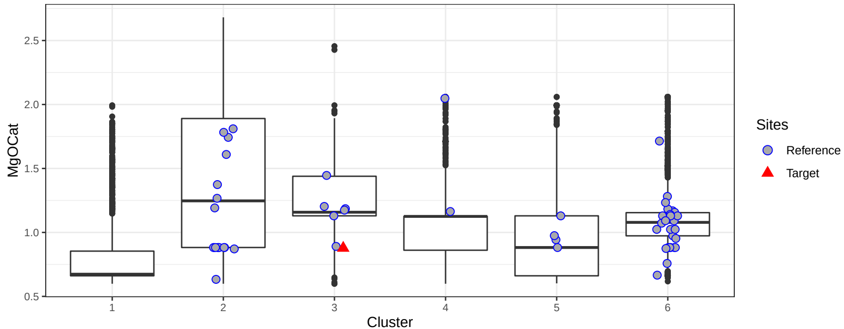
Surface MgO content (%) in the catchment by cluster
