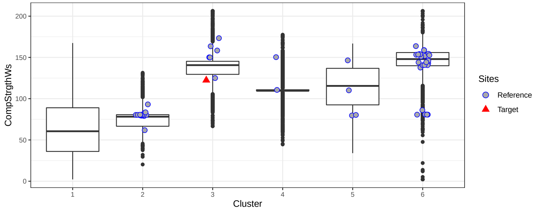
Compressive strength (megaPascals) in the watershed by cluster
