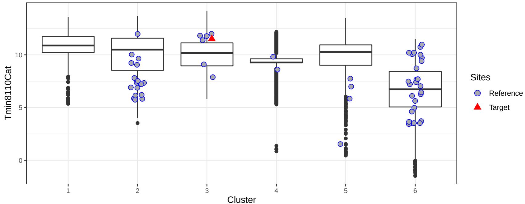
30-year normal minimum temperature (degrees C) in the catchment by cluster
