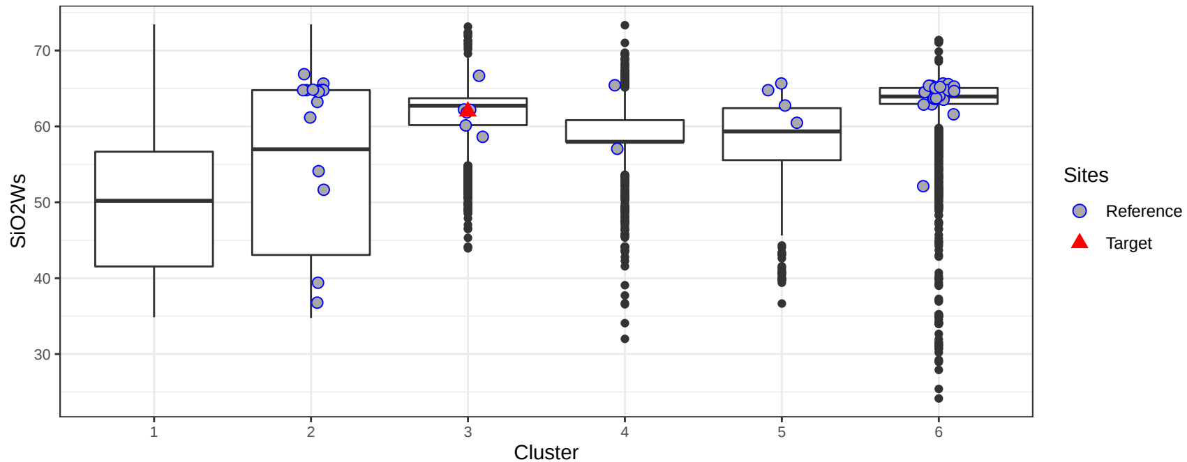
Surface SiO 2 content (%) in the watershed by cluster
