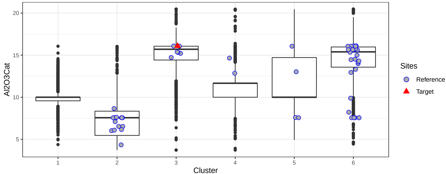
Surface Al 2 O 3 content (%) in the catchment by cluster
