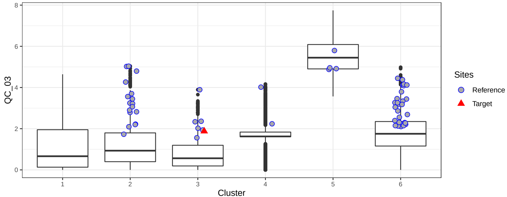
Mean March flow (est.) (cfs) in the catchment by cluster
