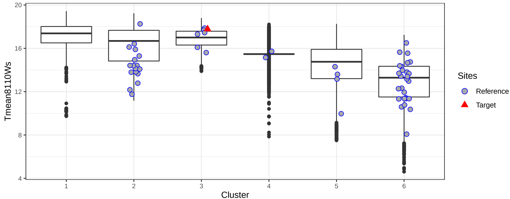
30-year normal mean temperature (degrees C) in the watershed by cluster
