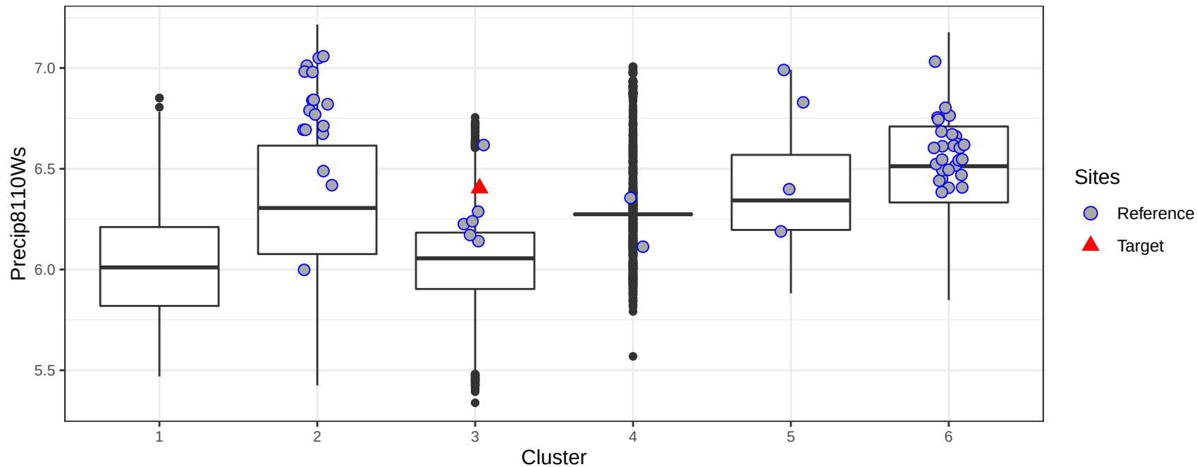
30-year normal mean precipitation (mm) in the watershed by cluster
