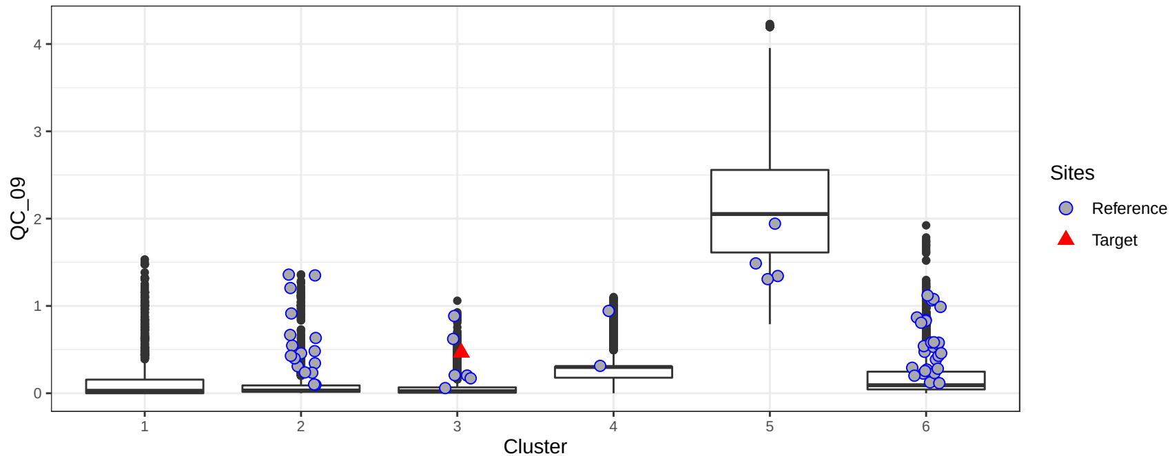
Mean September flow (est.) (cfs) in the catchment by cluster
