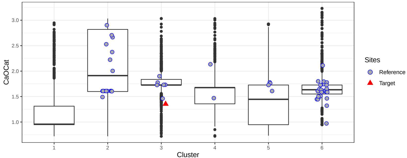
Surface CaO content (%) in the catchment by cluster
