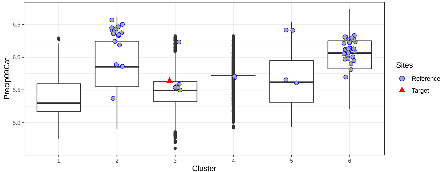
Mean precipitation in 2009 (mm) in the catchment by cluster
