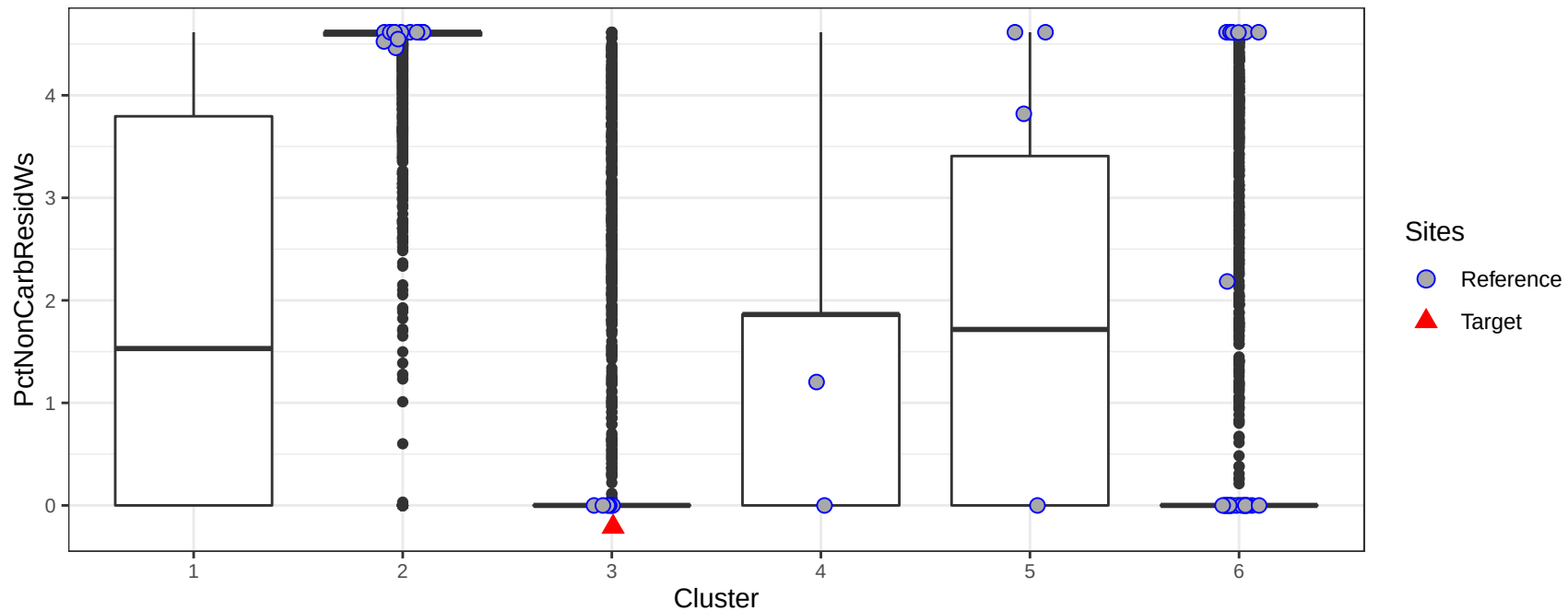
Non-carbonate residual material (%) in the watershed by cluster
