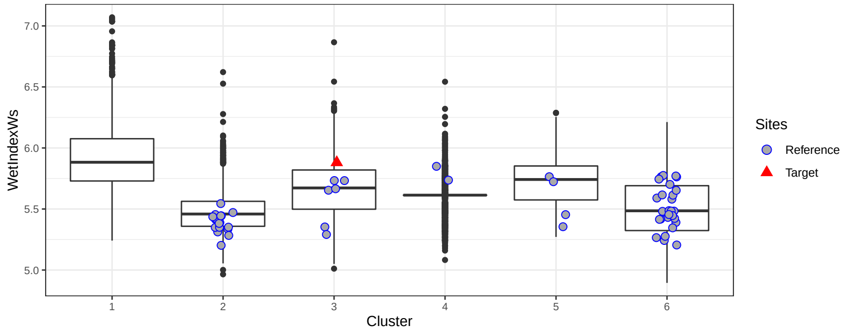
Wetness Index (unitless) in the watershed by cluster
