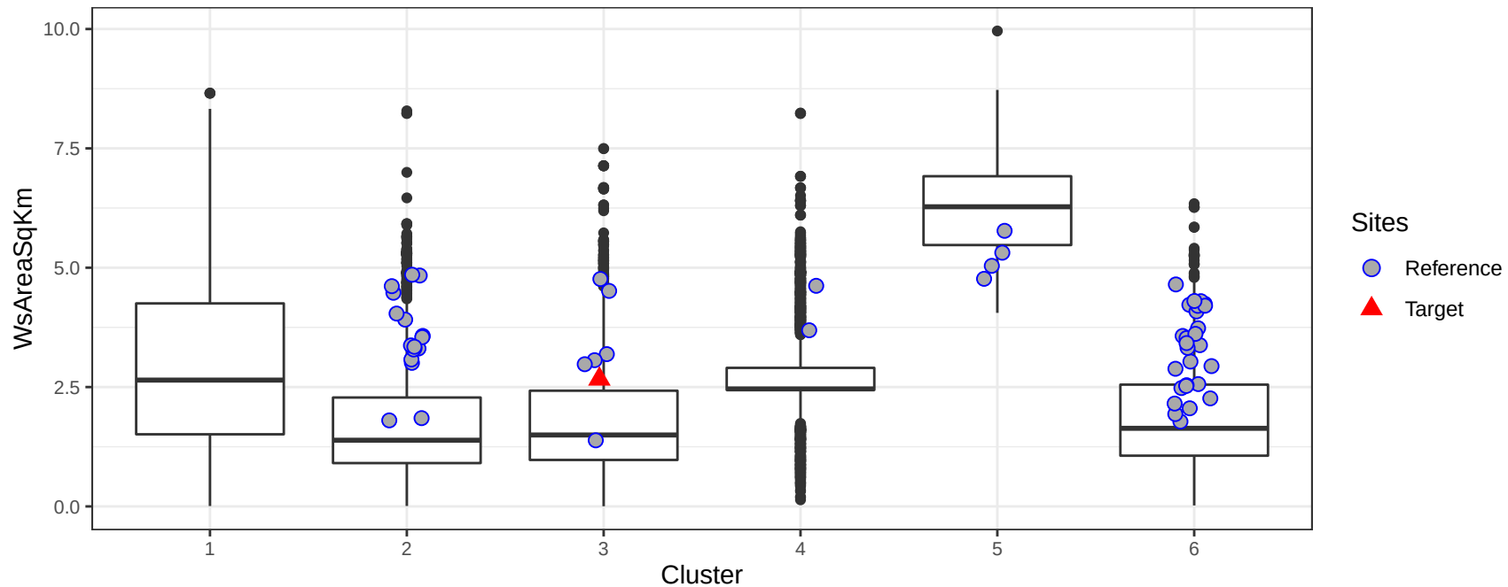
Drainage area (sq. km.) in the watershed by cluster
