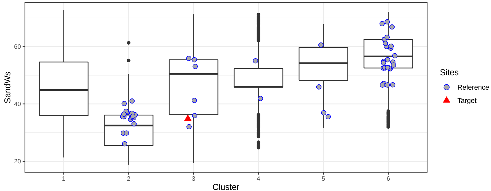
Mean sand content (%) in the watershed by cluster
