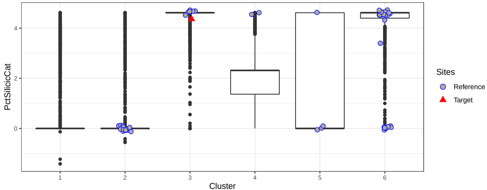
Silicic residual material (%) in the catchment by cluster
