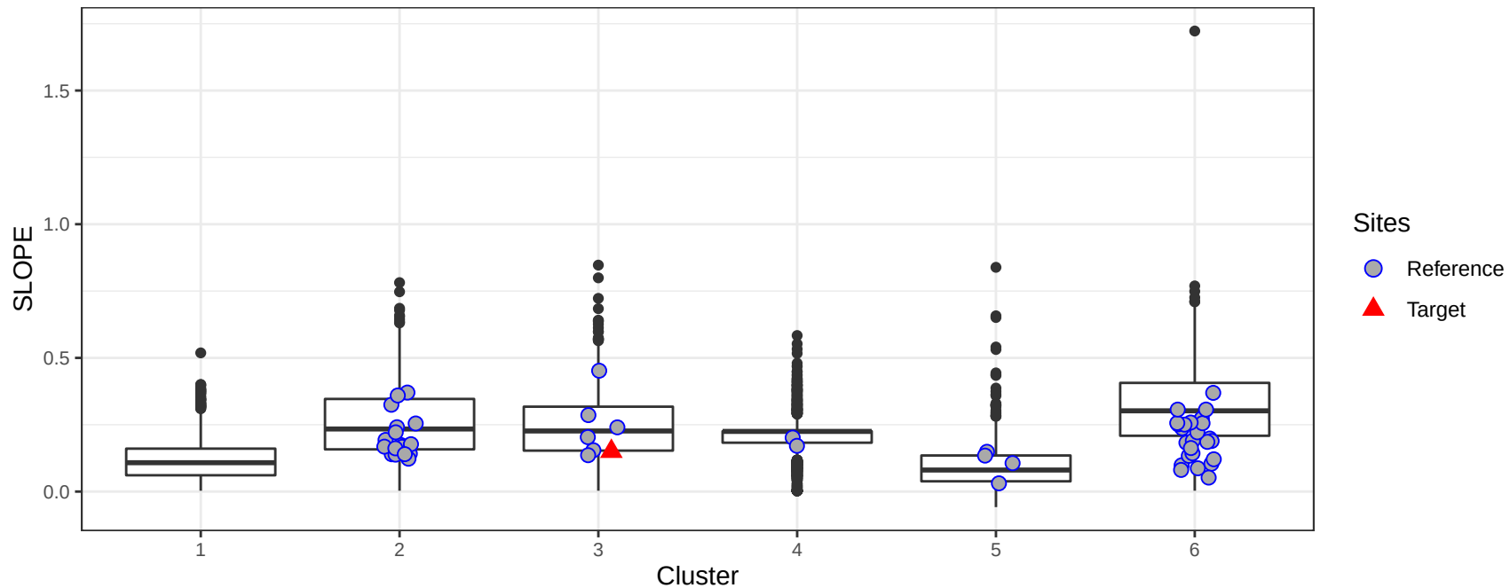
Slope (m/m) in the catchment by cluster
