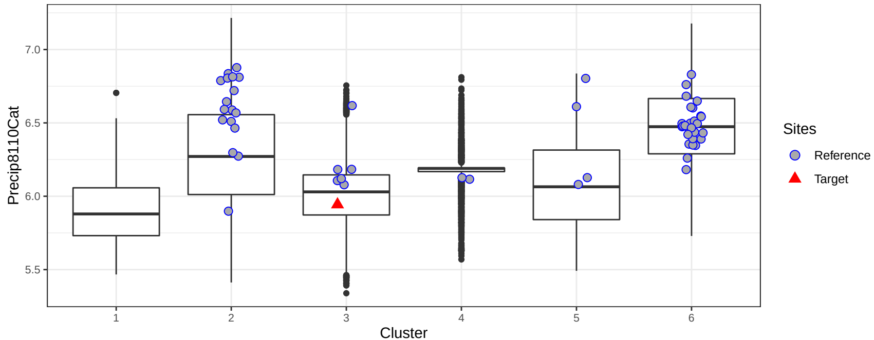
30-year normal mean precipitation (mm) in the catchment by cluster
