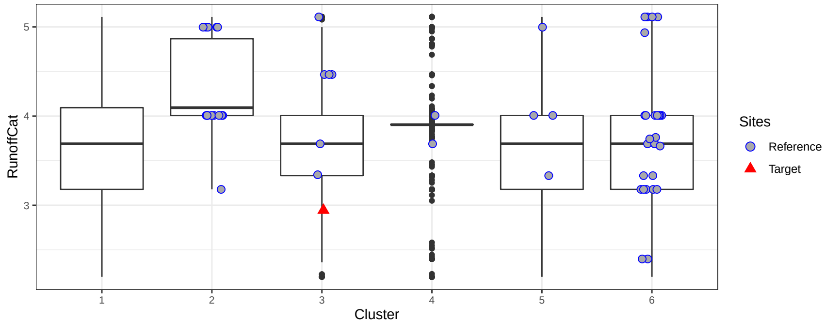
Mean runoff (mm) in the catchment by cluster
