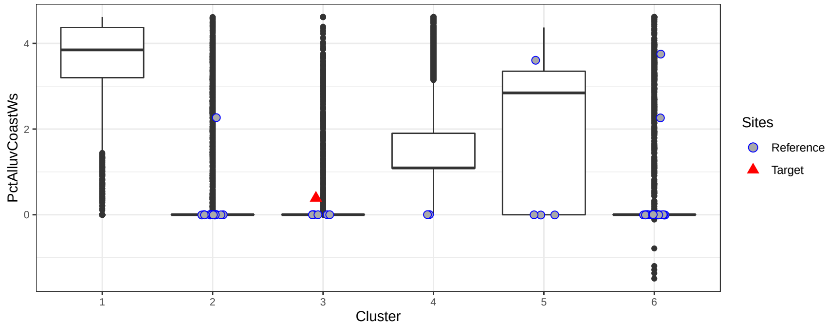
Alluvium and fine-textured coastal zone sediment (%) in the watershed by cluster
