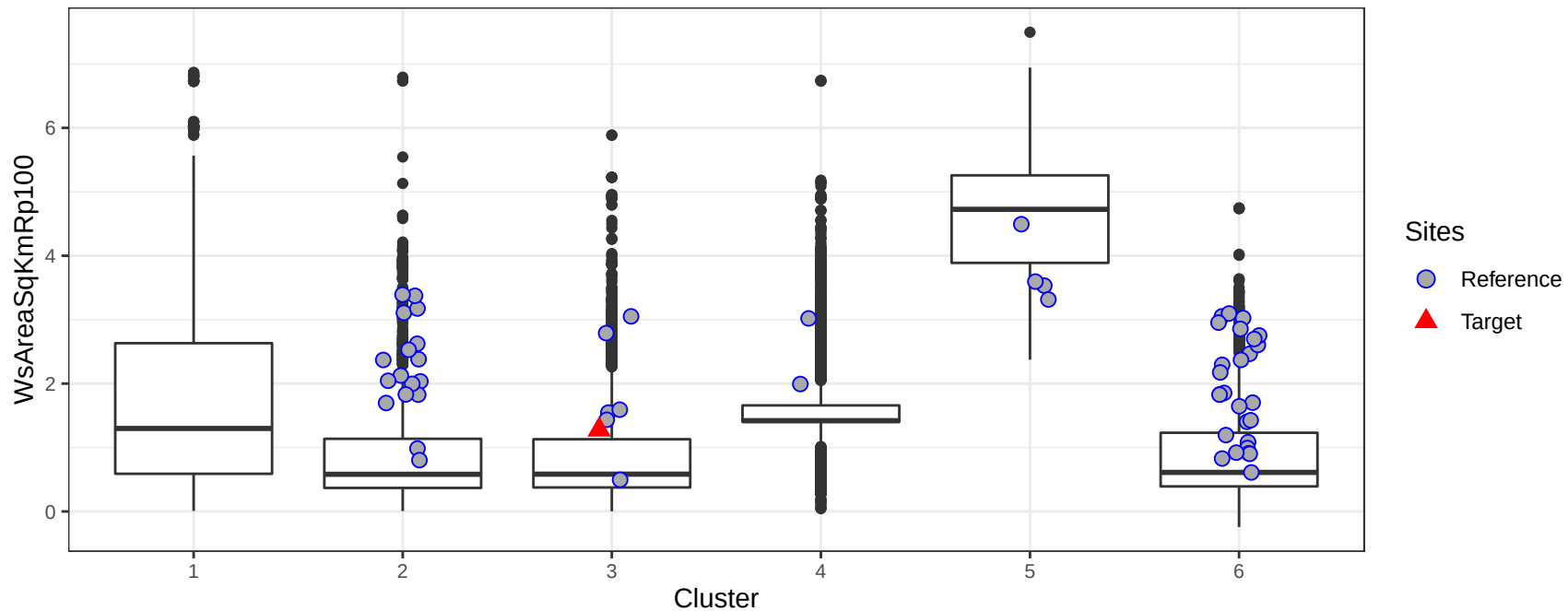
Area within the riparian buffer (sq. km.) in the watershed riparian by cluster
