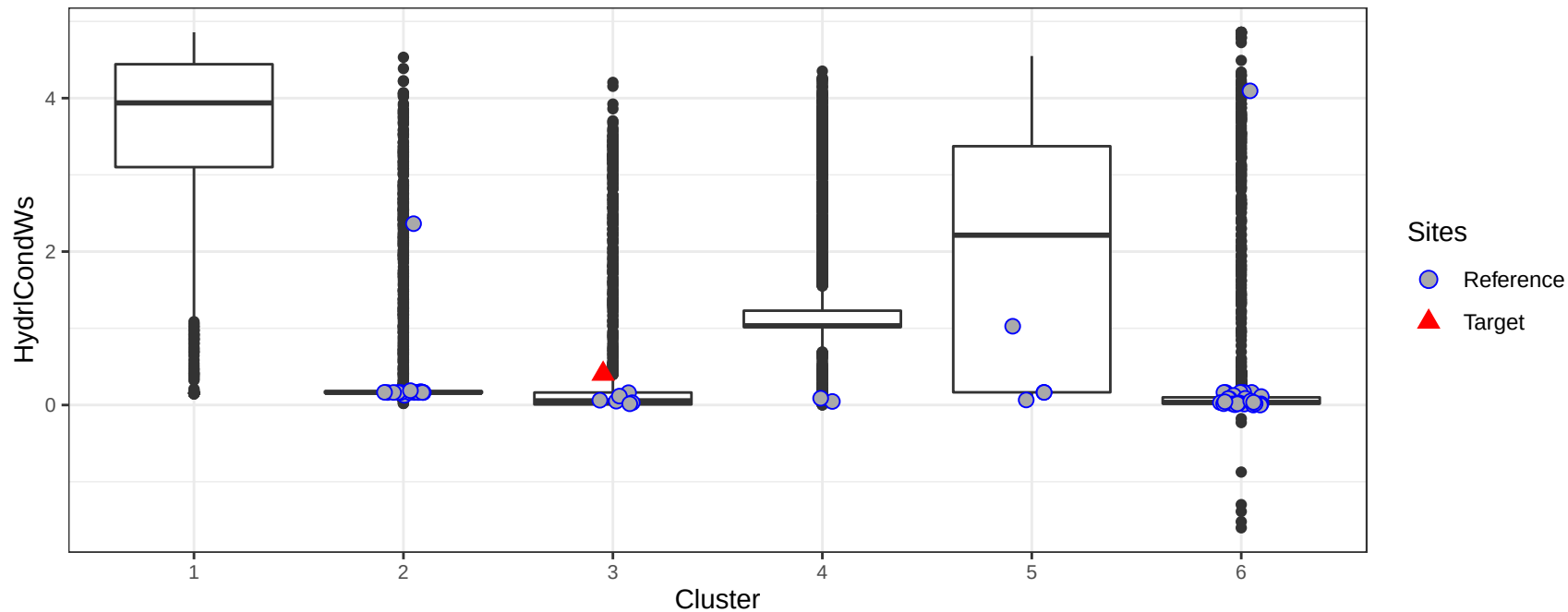
Hydraulic conductivity (um/sec) in the watershed by cluster
