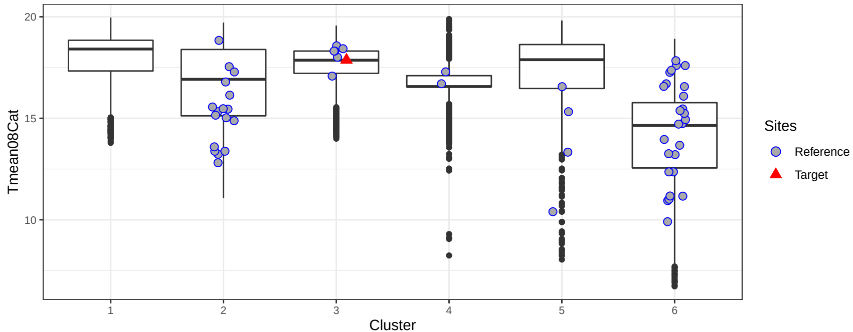
Mean temperature in 2008 (degrees C) in the catchment by cluster
