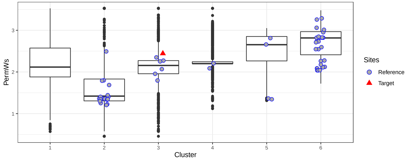
Mean permeability (cm/hr) in the watershed by cluster
