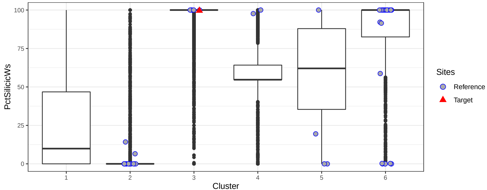
Silicic residual material (%) in the watershed by cluster
