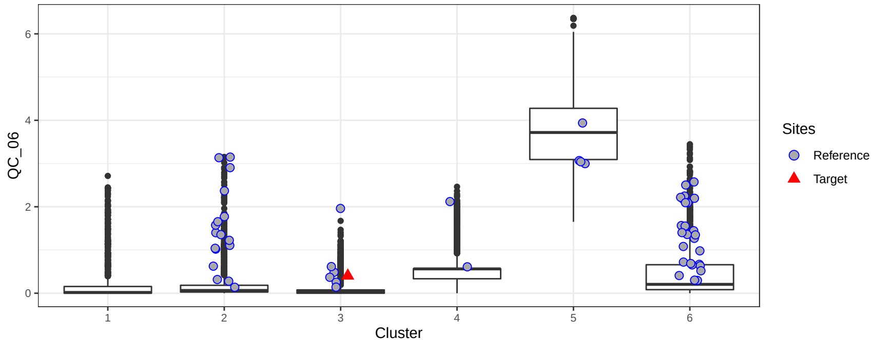
Mean June flow (est.) (cfs) in the catchment by cluster
