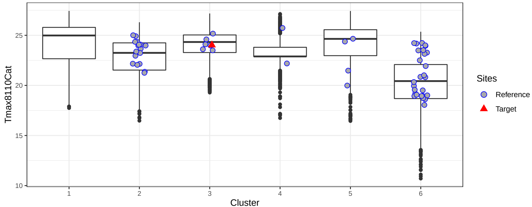
30-year normal maximum temperature (degrees C) in the catchment by cluster
