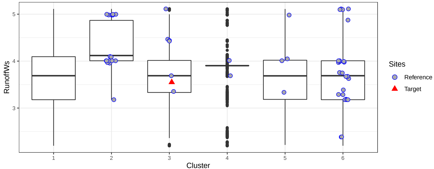
Mean runoff (mm) in the watershed by cluster
