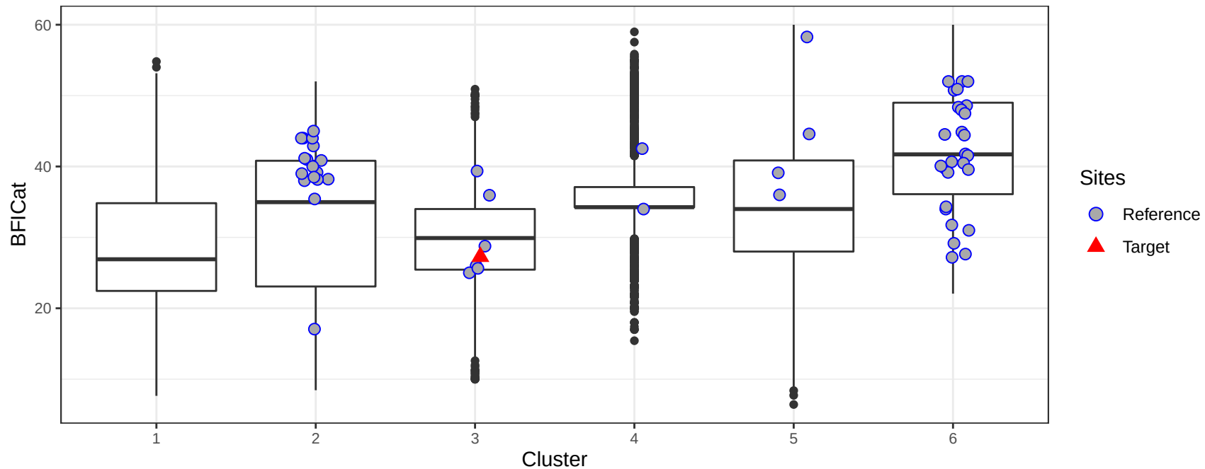
Base flow: total flow ratio (%) in the catchment by cluster
