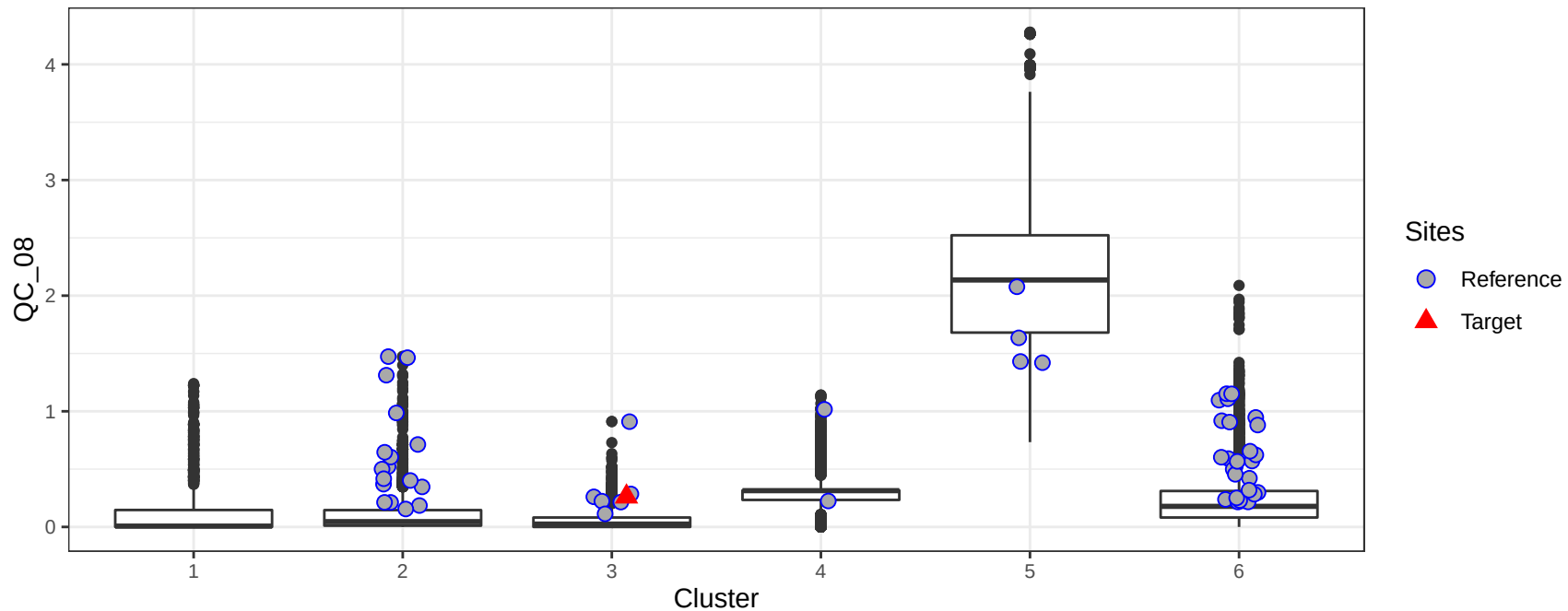
Mean August flow (est.) (cfs) in the catchment by cluster
