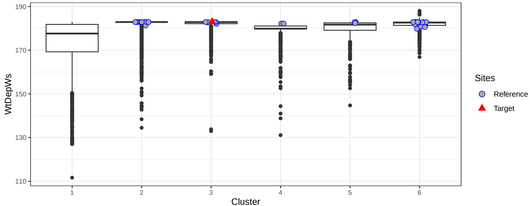
Mean seasonal water table depth (cm/hr) in the watershed by cluster
