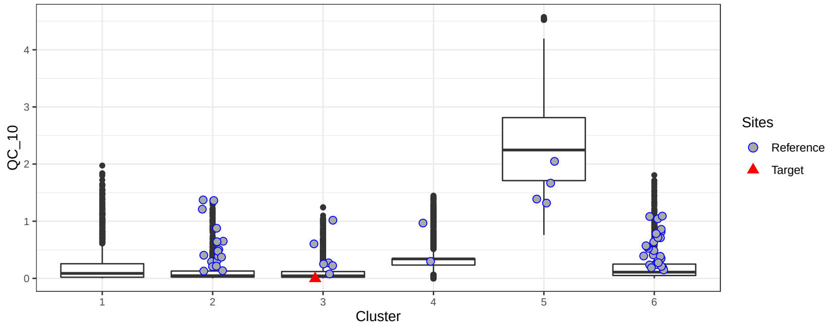
Mean October flow (est.) (cfs) in the catchment by cluster
