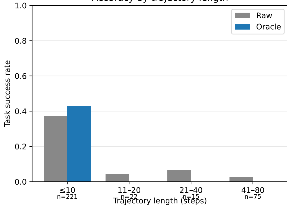
Accuracy by trajectory length
