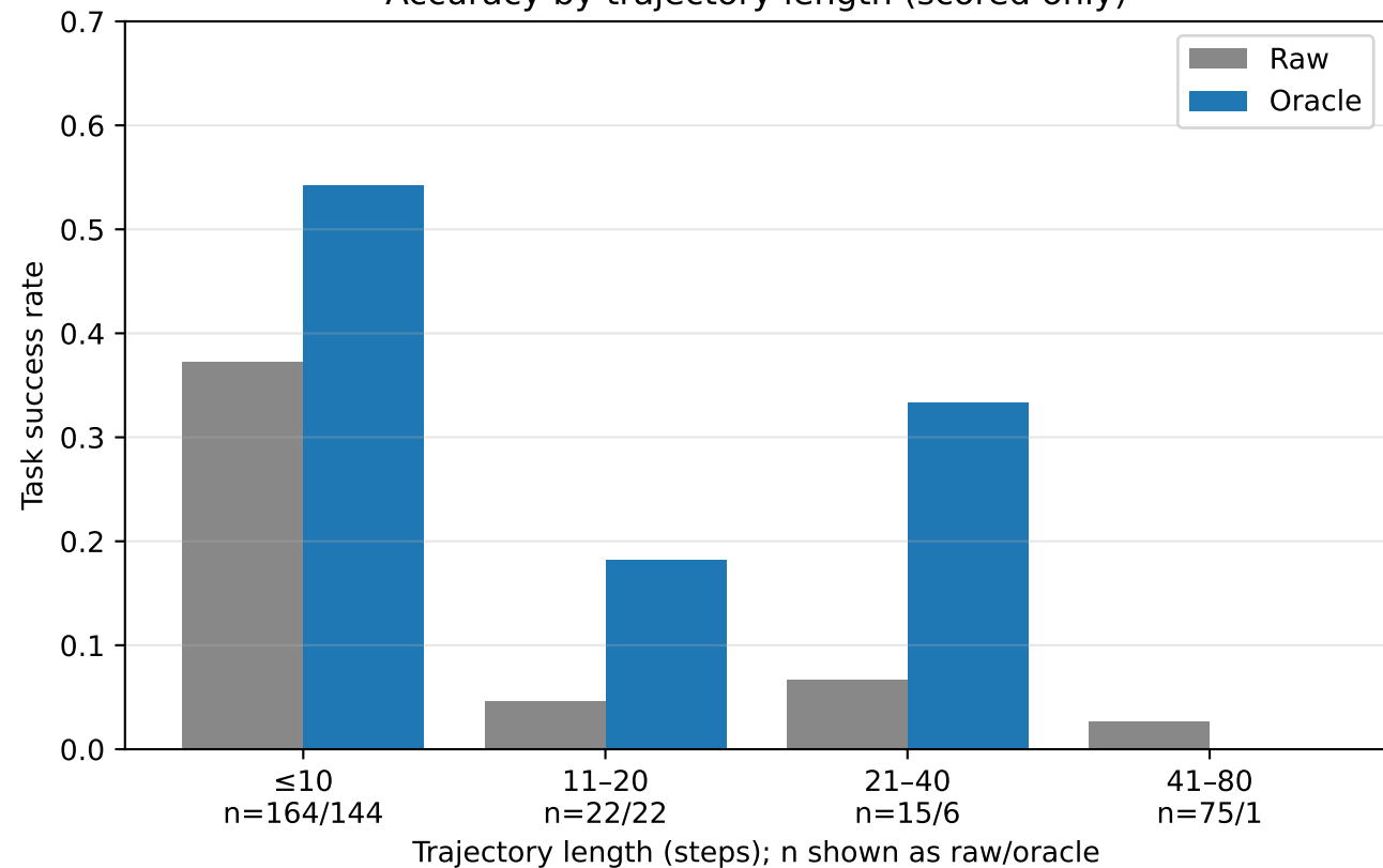
Accuracy by trajectory length (scored only)
