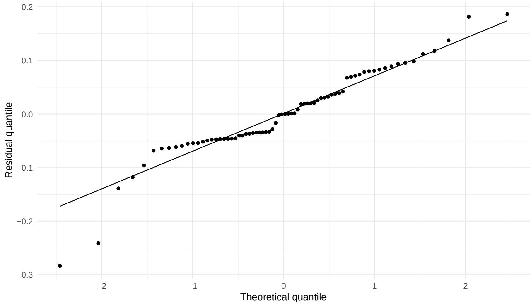
Historical-model residual normality
