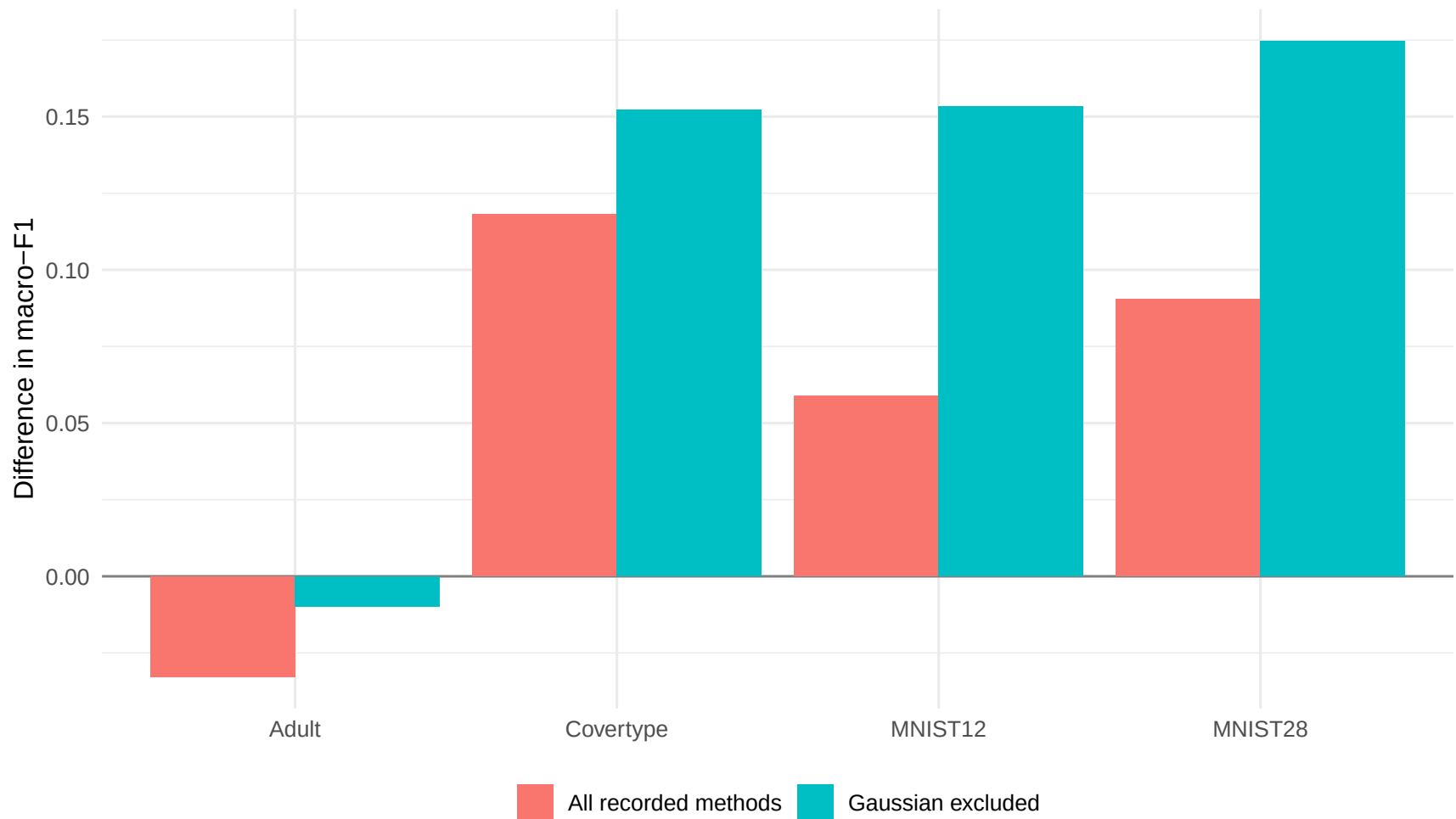
Decoupled minus joint generation by dataset
