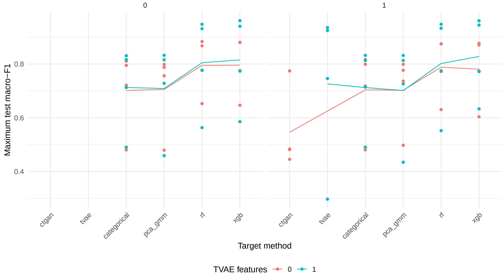
Labeler scores by feature generator and target inclusion
