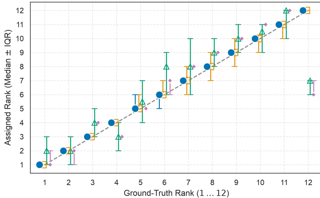
(B1) Assigned Rank vs. Ground Truth: Independent Criteria ( \rho = 0.0 )
