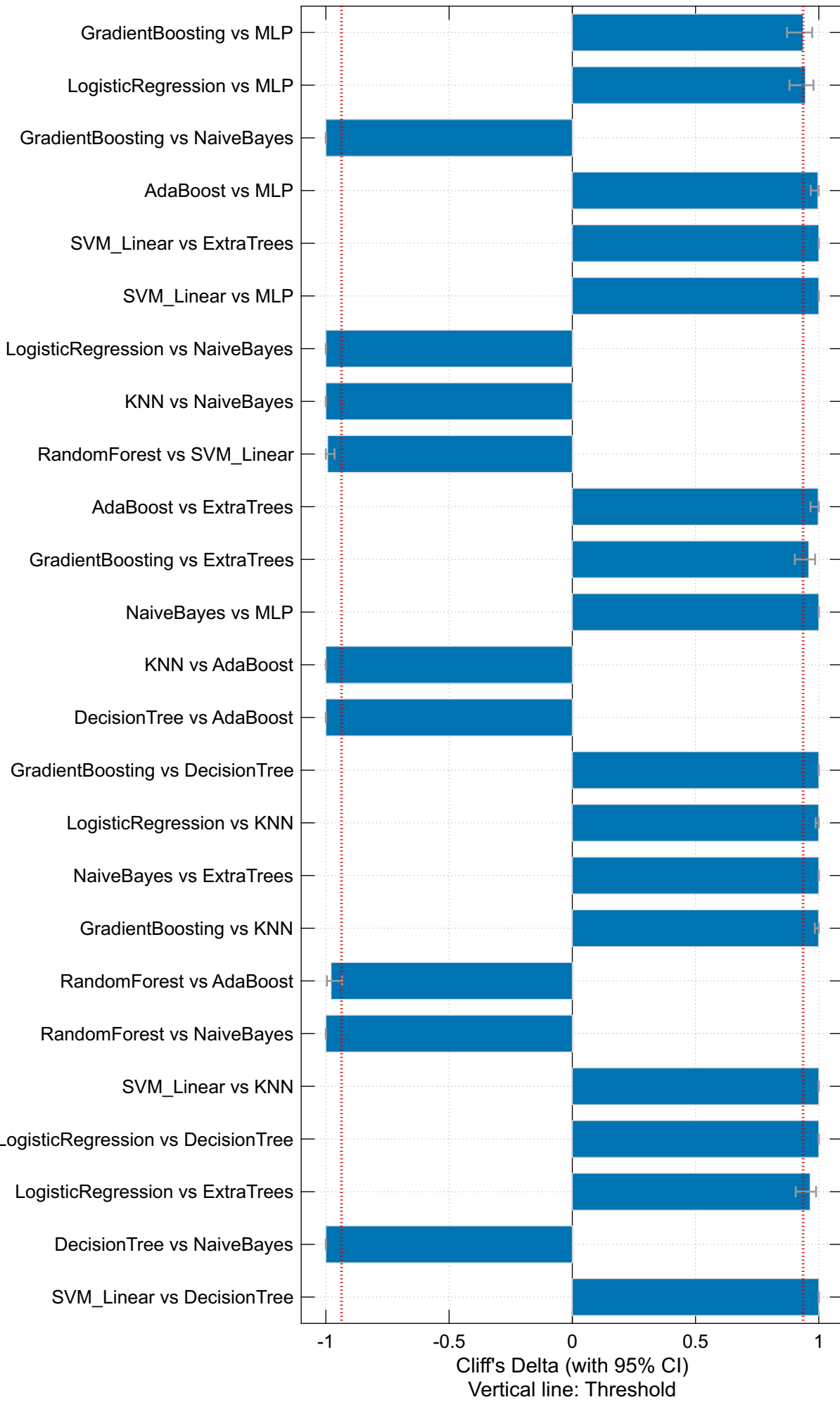
Effect Size Cliff's Delta
