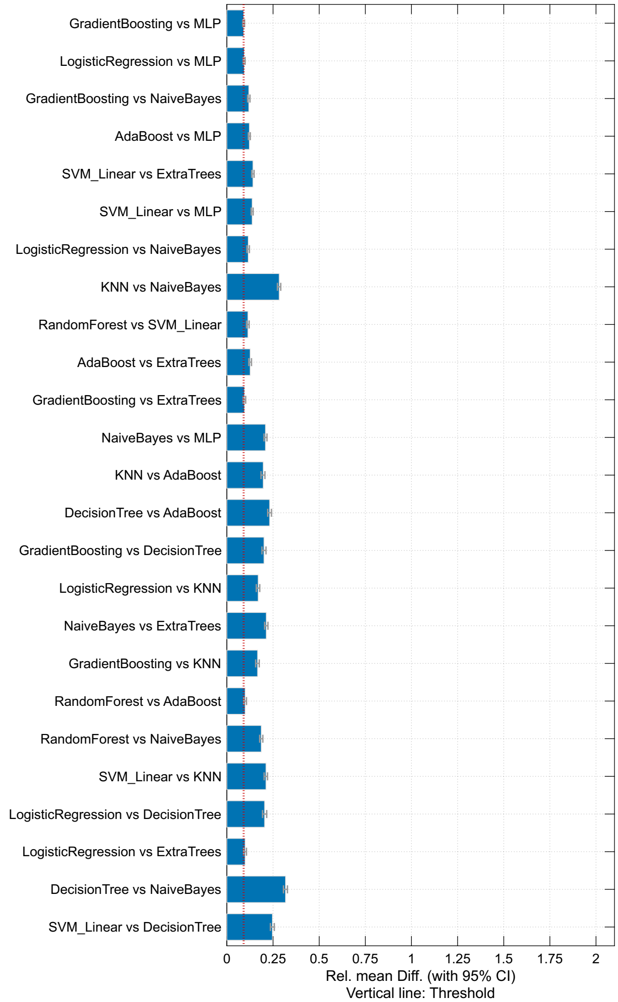
Relative Mean Difference
