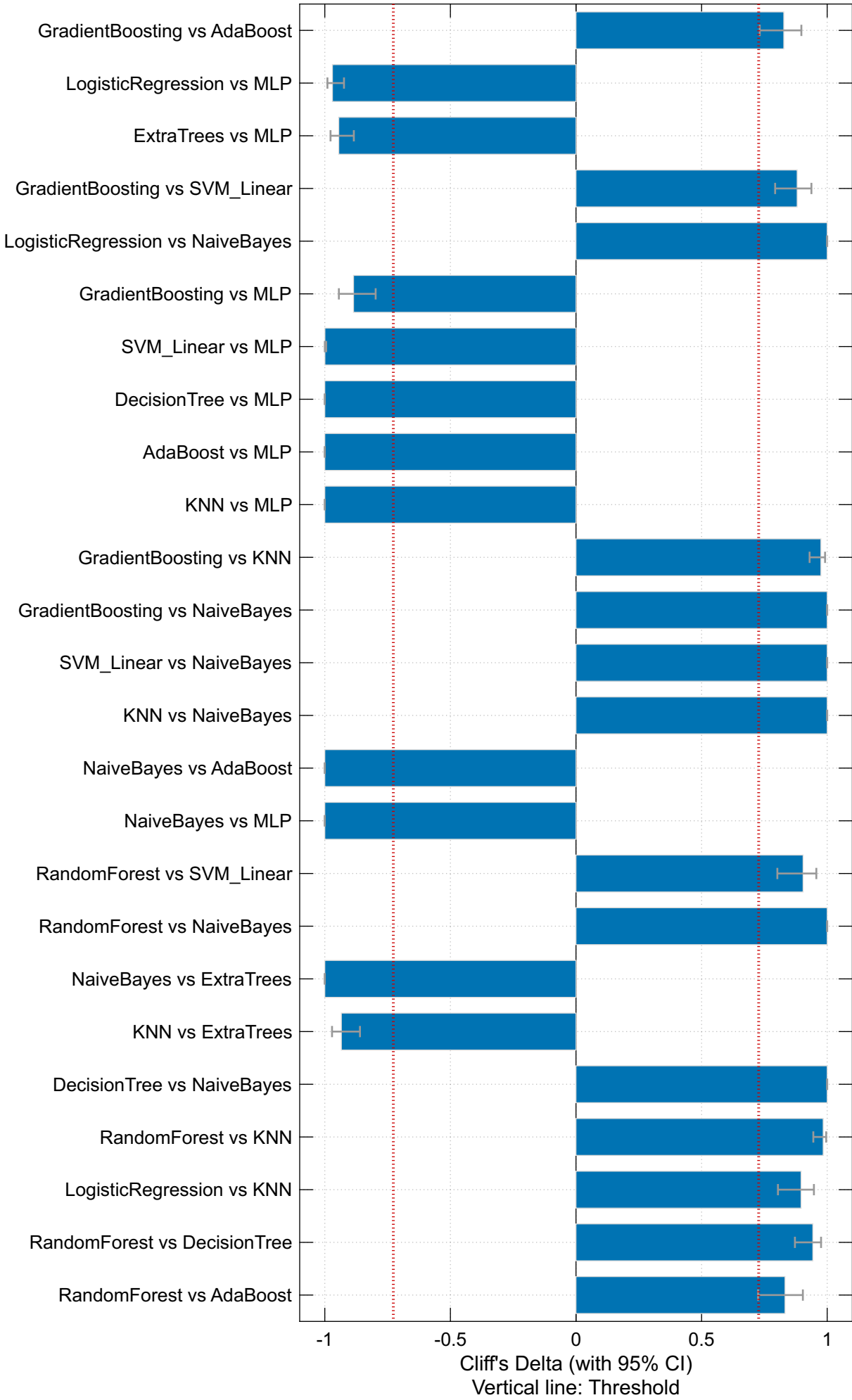
Effect Size Cliff's Delta
