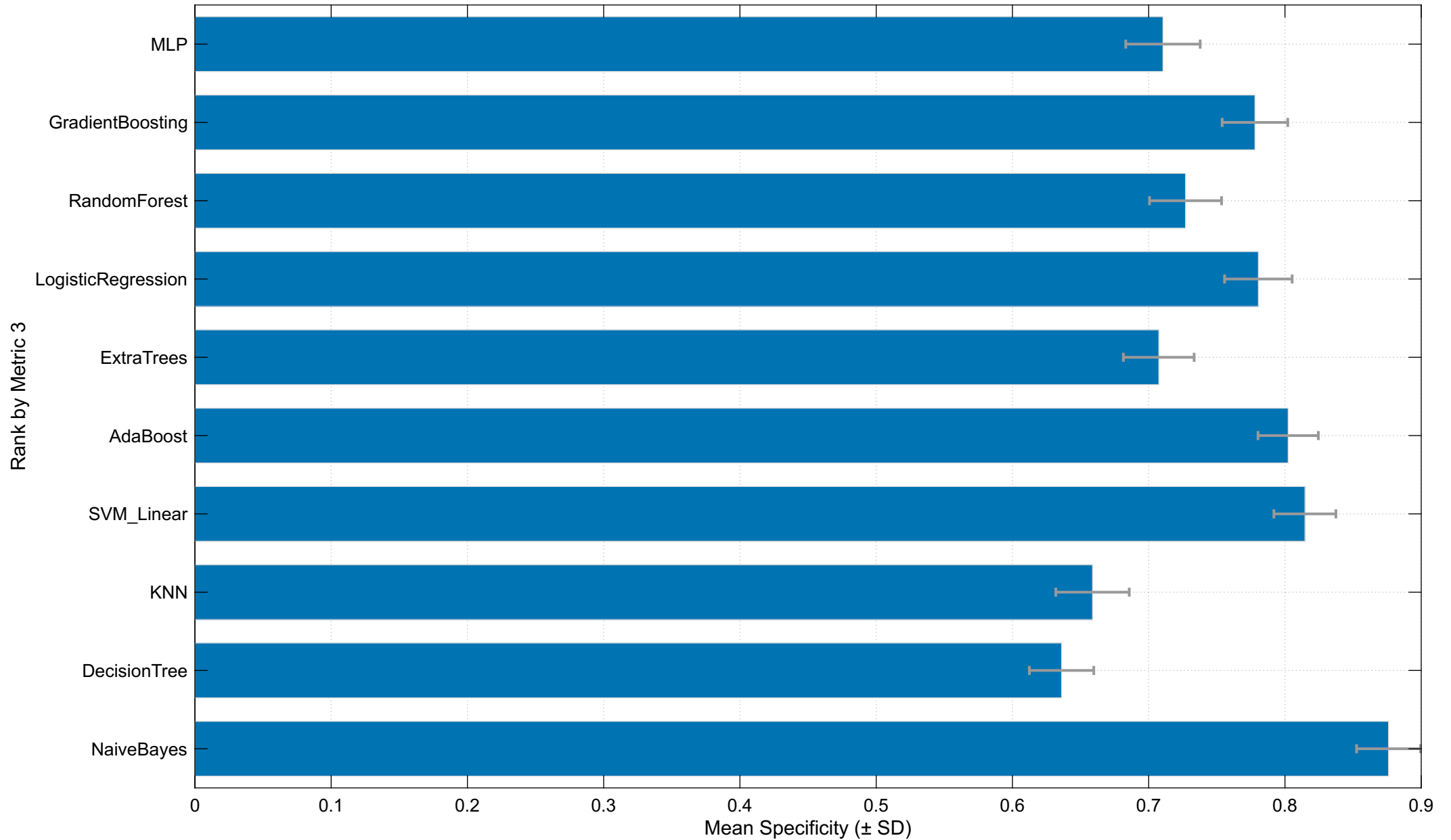
Ranking after Specificity Correction
