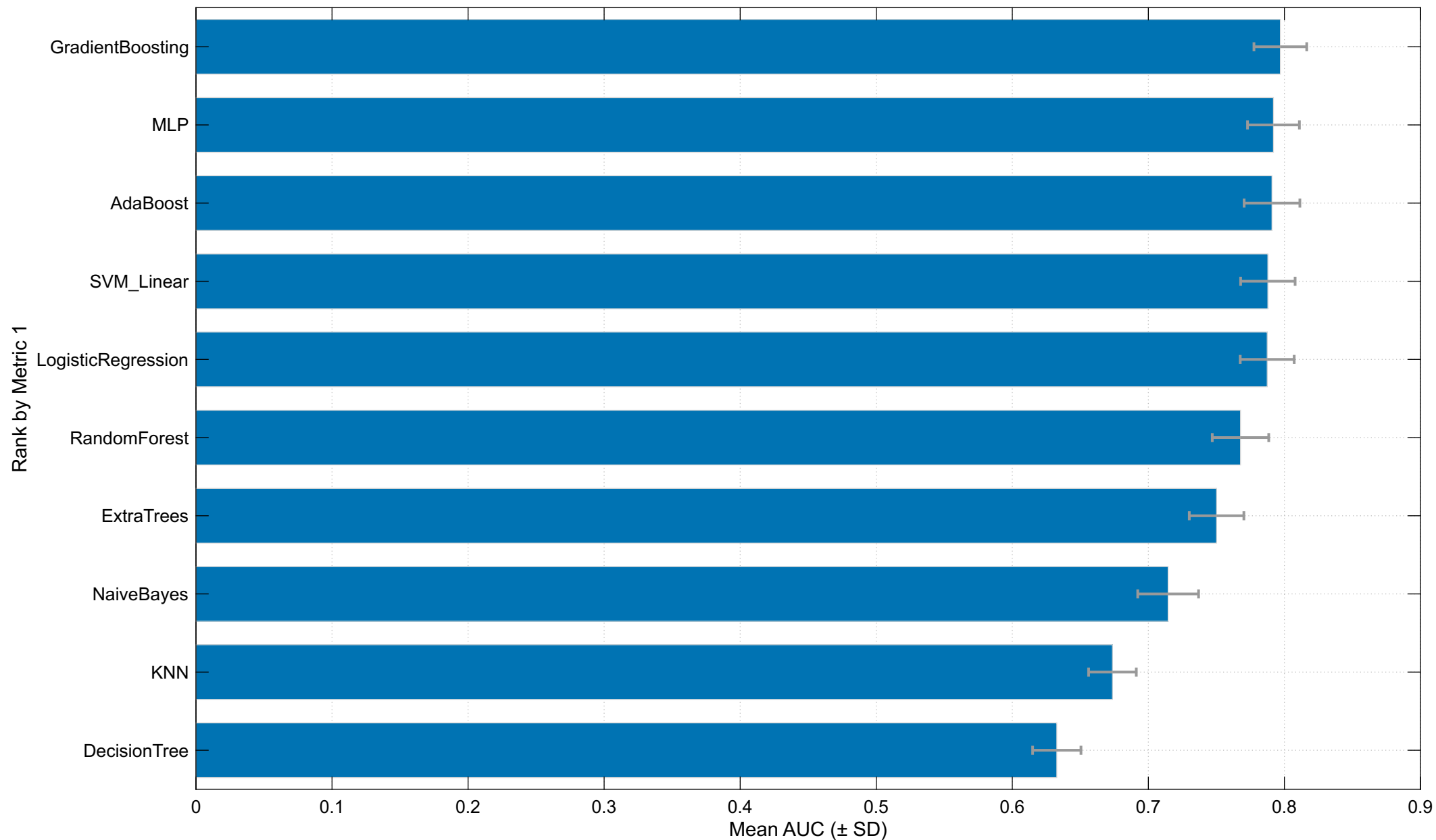
Ranking by AUC
