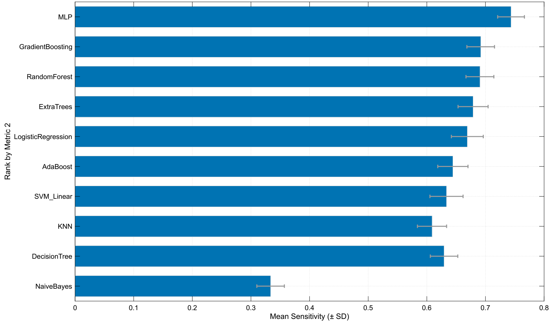
Ranking after Sensitivity Correction
