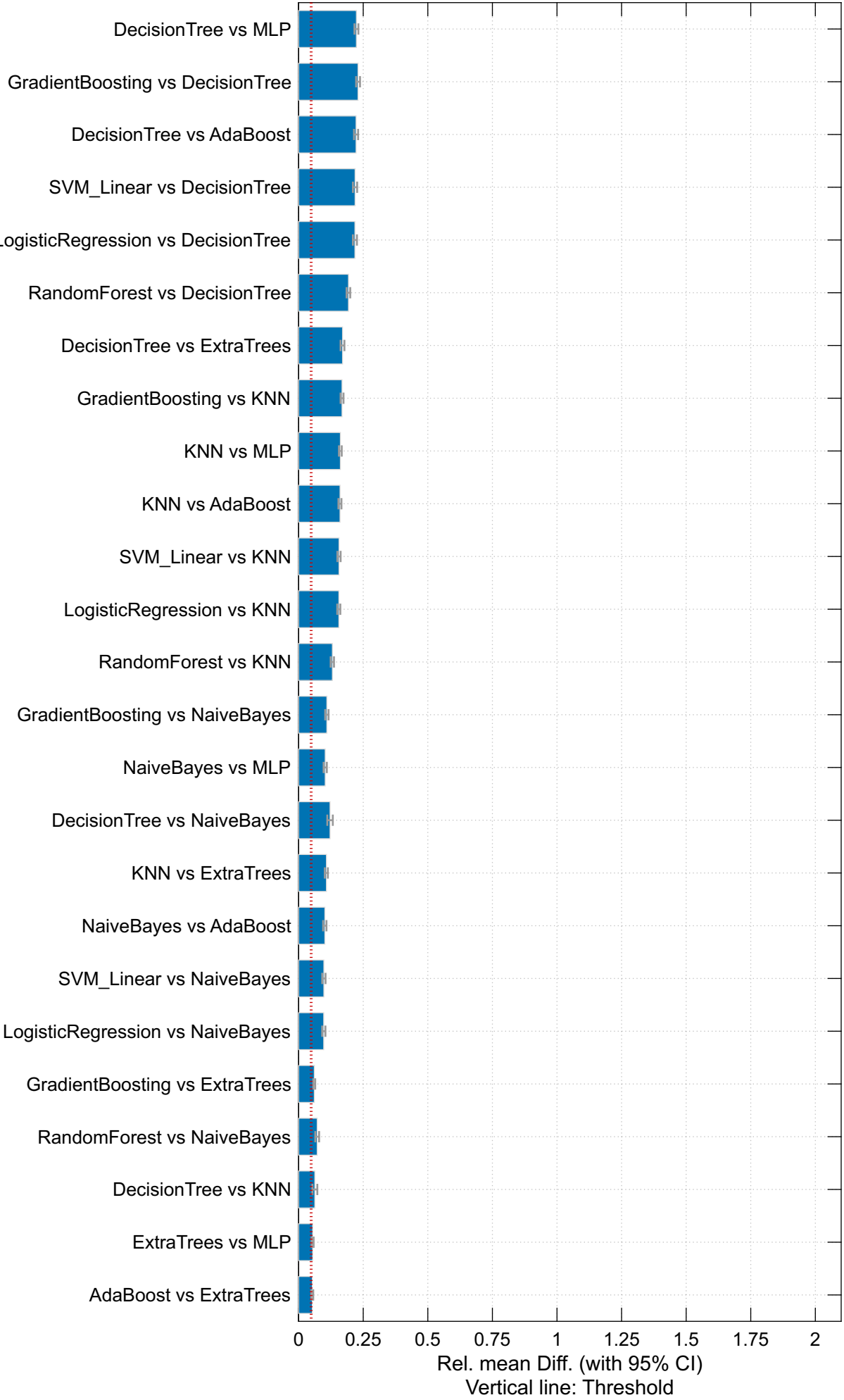
Relative Mean Difference
