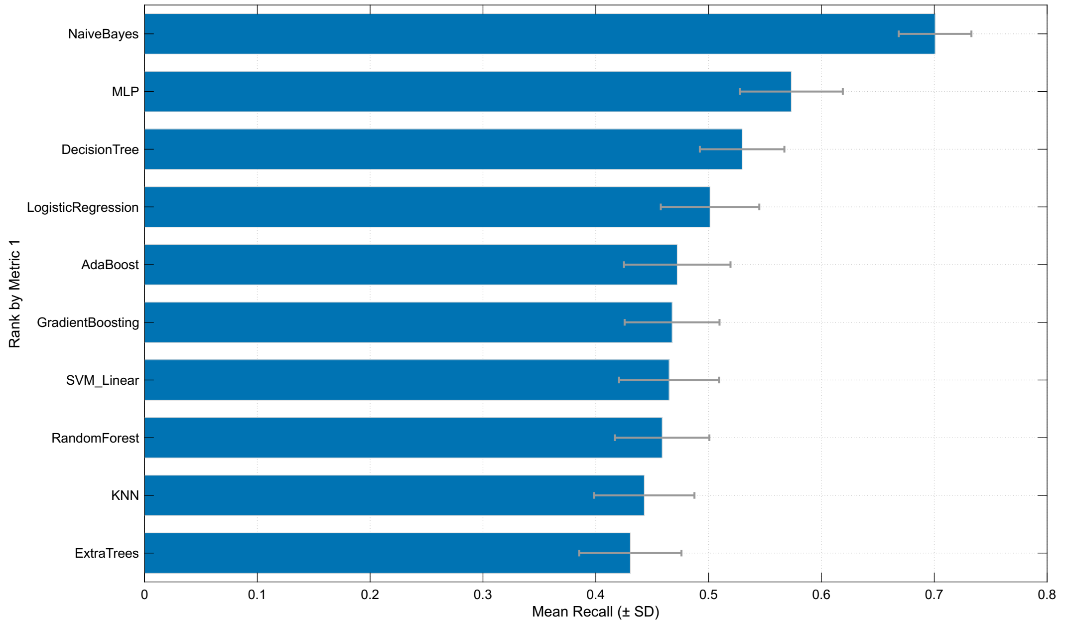
Ranking by Recall
