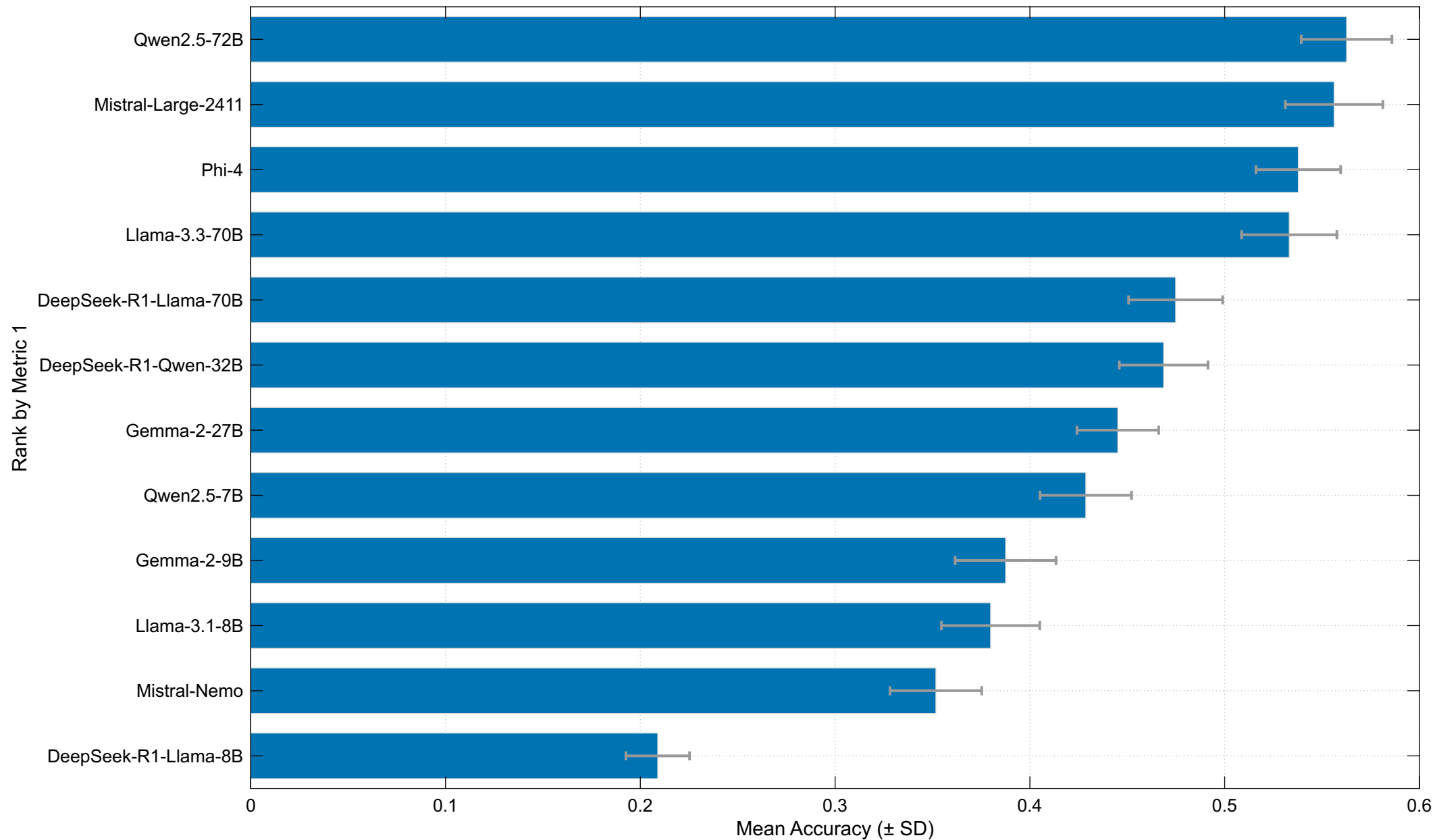
Ranking by Accuracy
