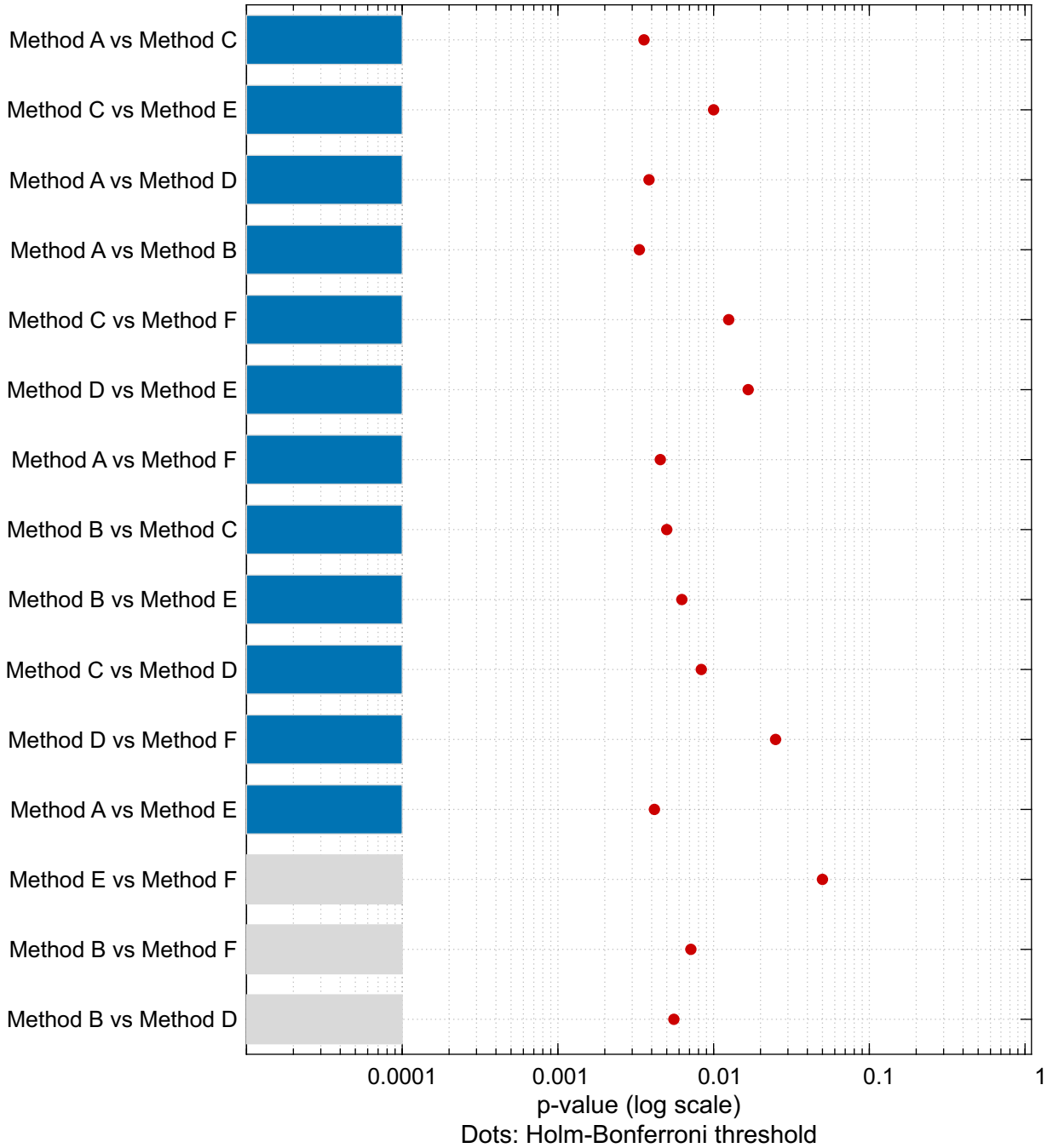
Statistical Significance
