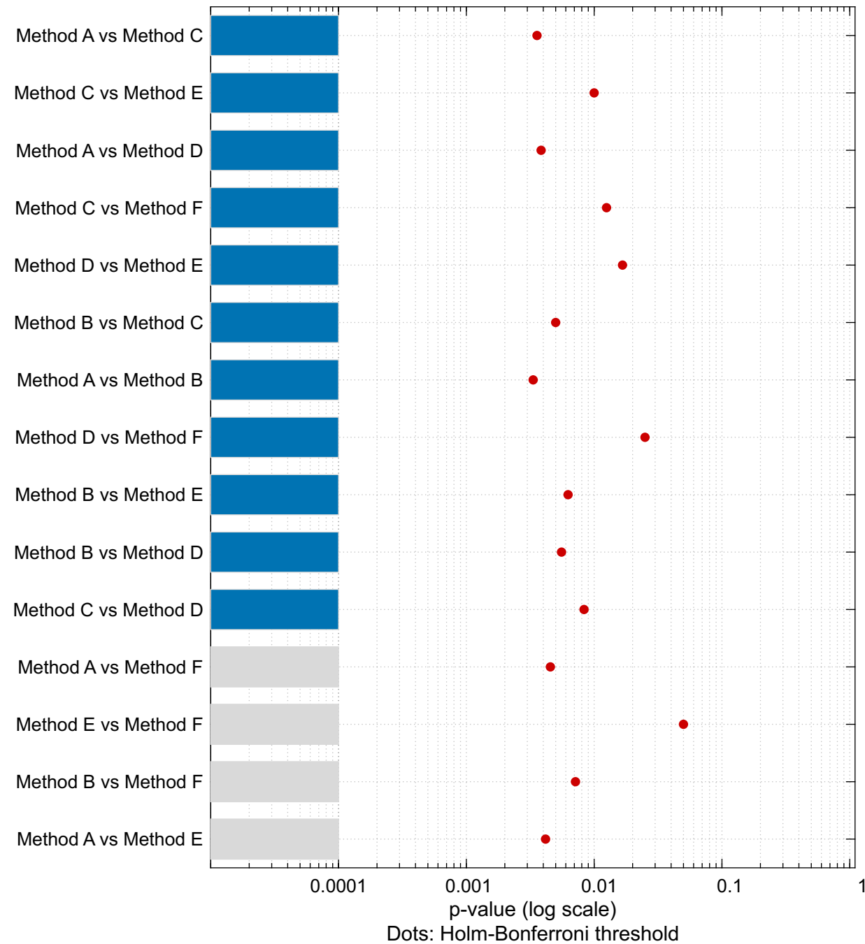
Statistical Significance
