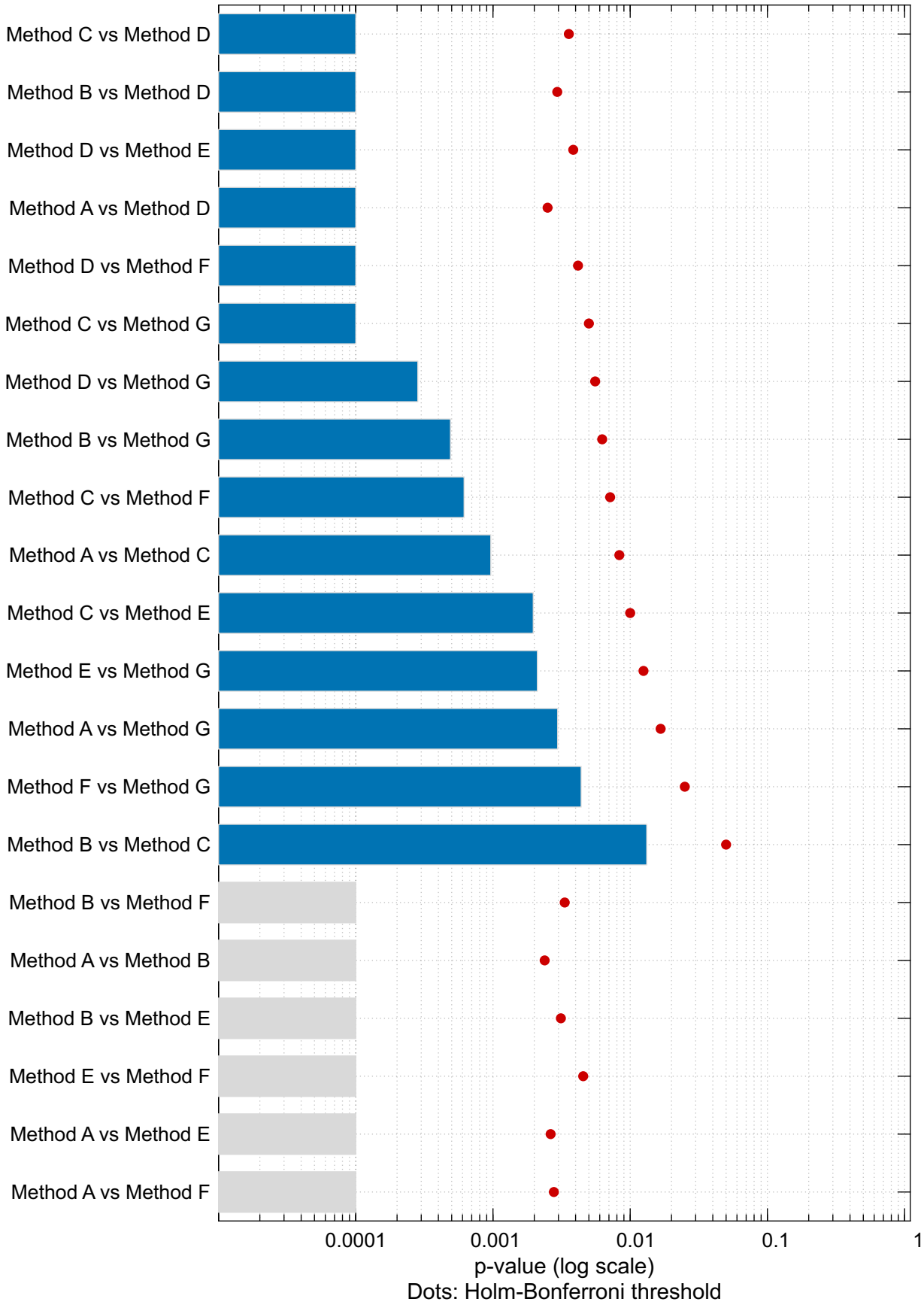
Statistical Significance
