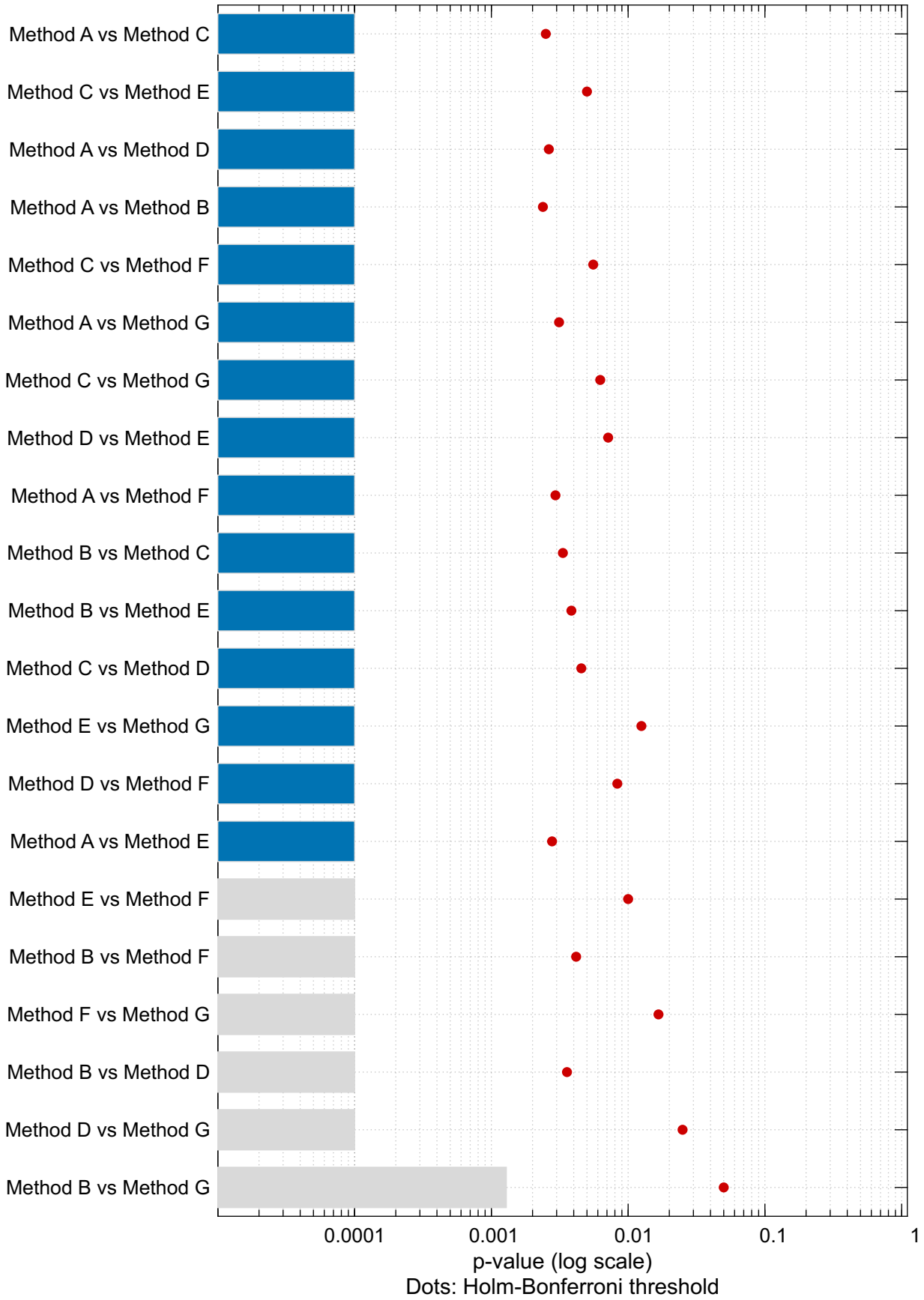
Statistical Significance
