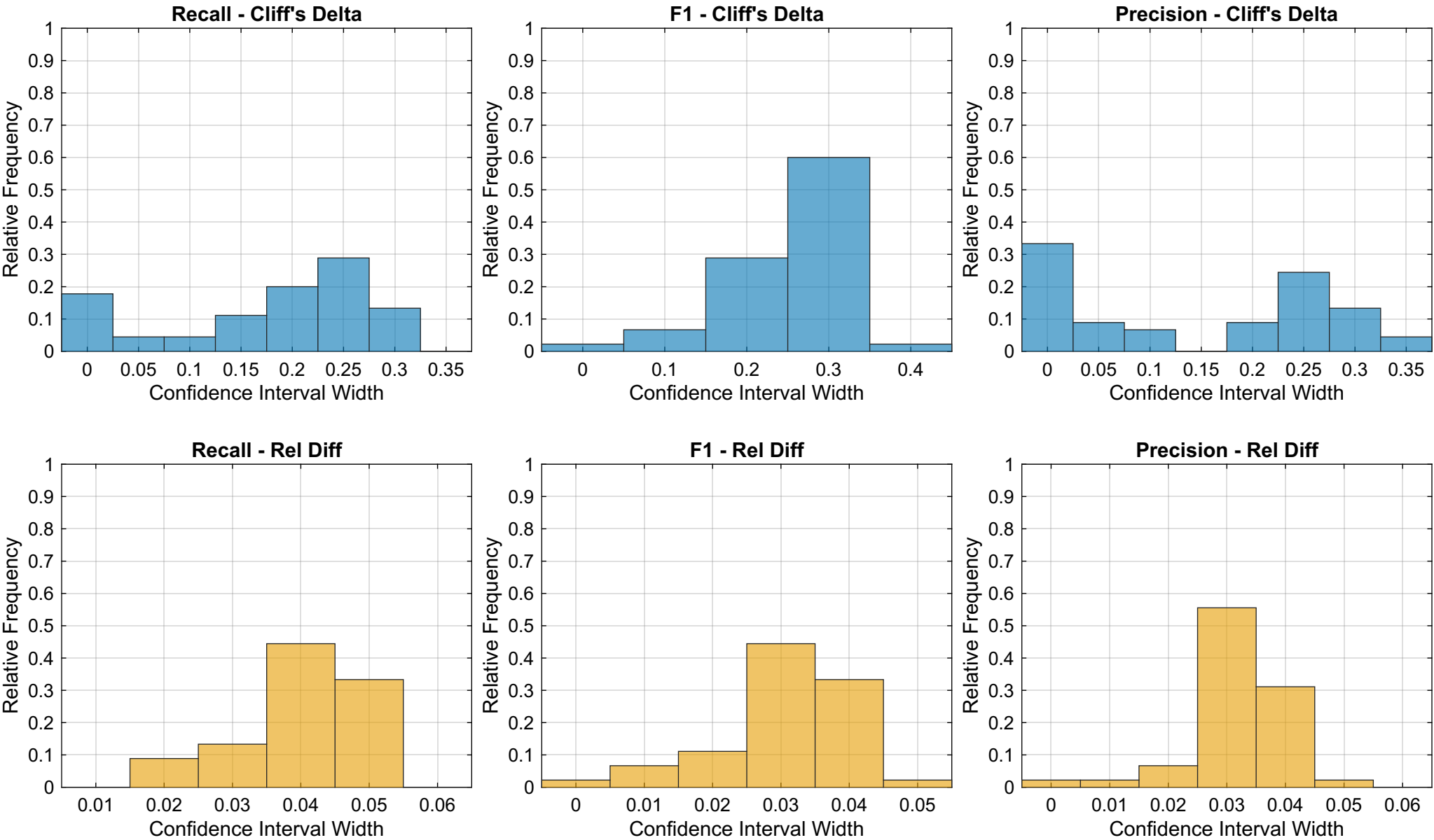
Distribution of Confidence Interval Widths across 45 pairwise comparisons (B = 4300)
