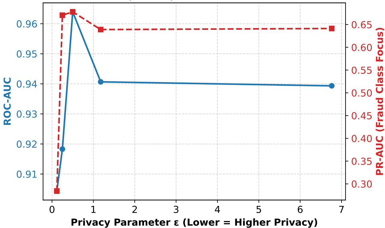
DP-SGD Utility-Privacy Trade-off (Credit Card Fraud)
