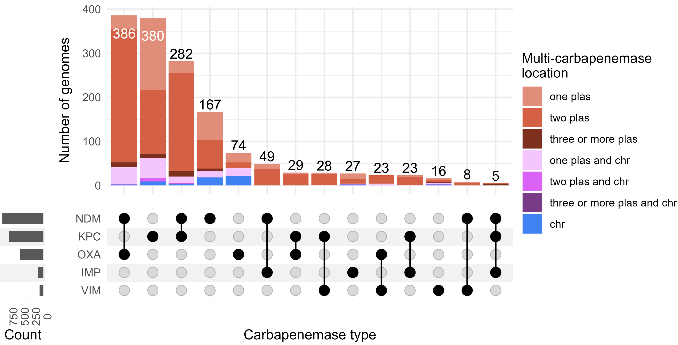
Figure 1: Most common carbapenemase combinations coloured by genomic location. “Plas” = plasmid, “chr” = chromosome.
