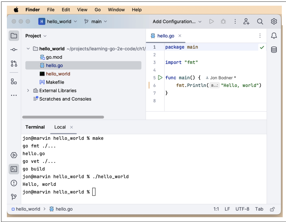
Figure 1-2. GoLand
