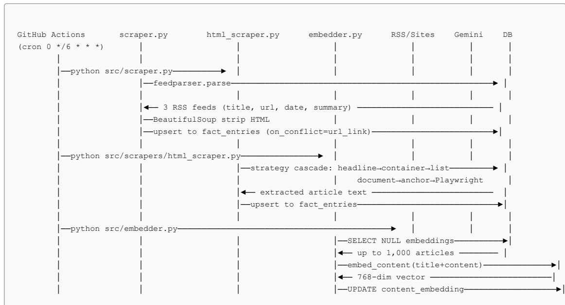
Figure 4.4 — Automated Ingestion Pipeline Sequence
