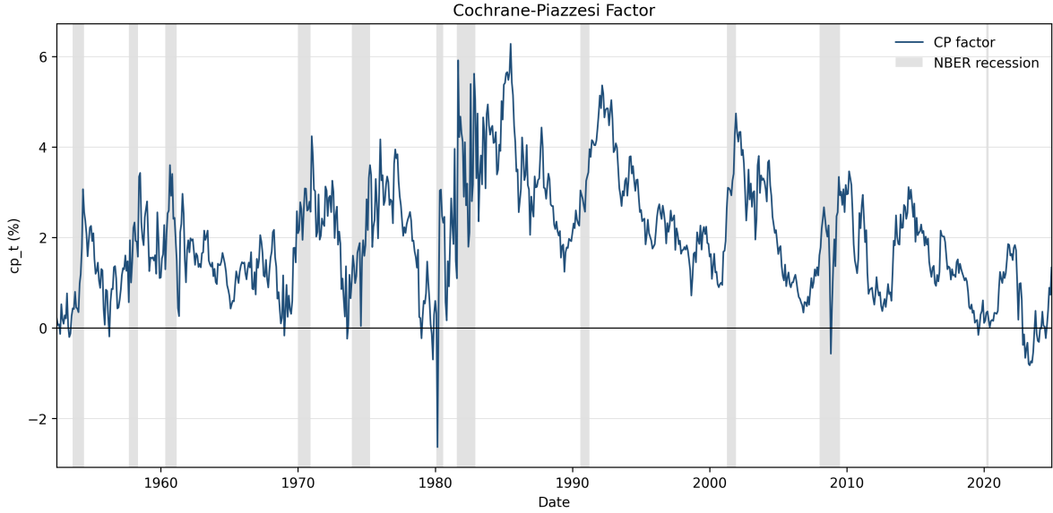
Figure 17: Cochrane–Piazzesi factor with NBER recession periods.
