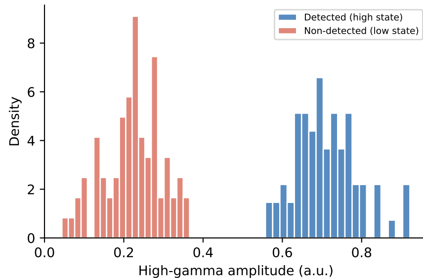
Pred 5.a — Frontoparietal bimodal distribution
