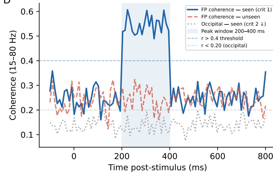
Pred 5.d — Gamma coherence predicts detection (1+2=GNW; +HEP-coh r > 0.25 = APGI)
