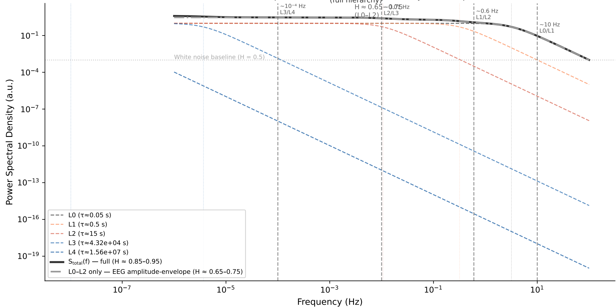
Figure 2 — 1/f Power Spectrum from OU Superposition Five Lorentzians + Composite + Partial-Hierarchy Overlay (§2.4, Paper 3)
