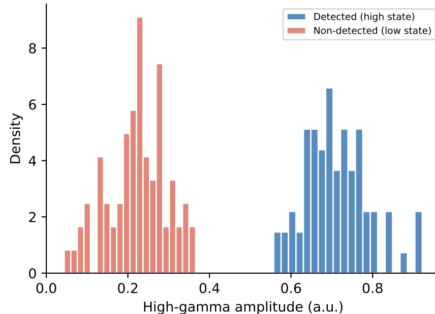
Pred 6.a — Frontoparietal bimodal distribution
