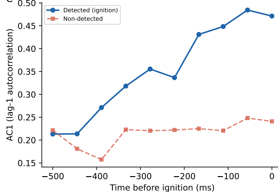
Pred 6.c — Critical slowing: AC1 \uparrow before ignition (APGI vs. GWT criterion)
