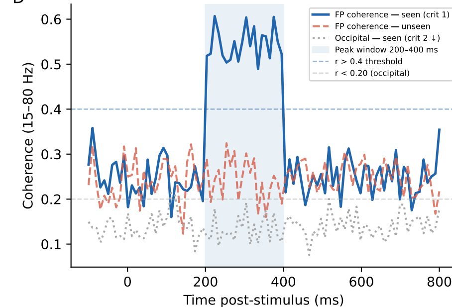
Pred 6.d — Gamma coherence predicts detection (1+2=GNW; +HEP-coh r > 0.25 = APGI)
