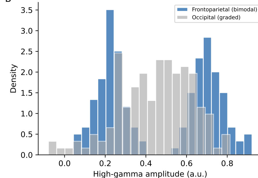
Pred 6.b — Regional specificity: FP bimodal, occipital graded
