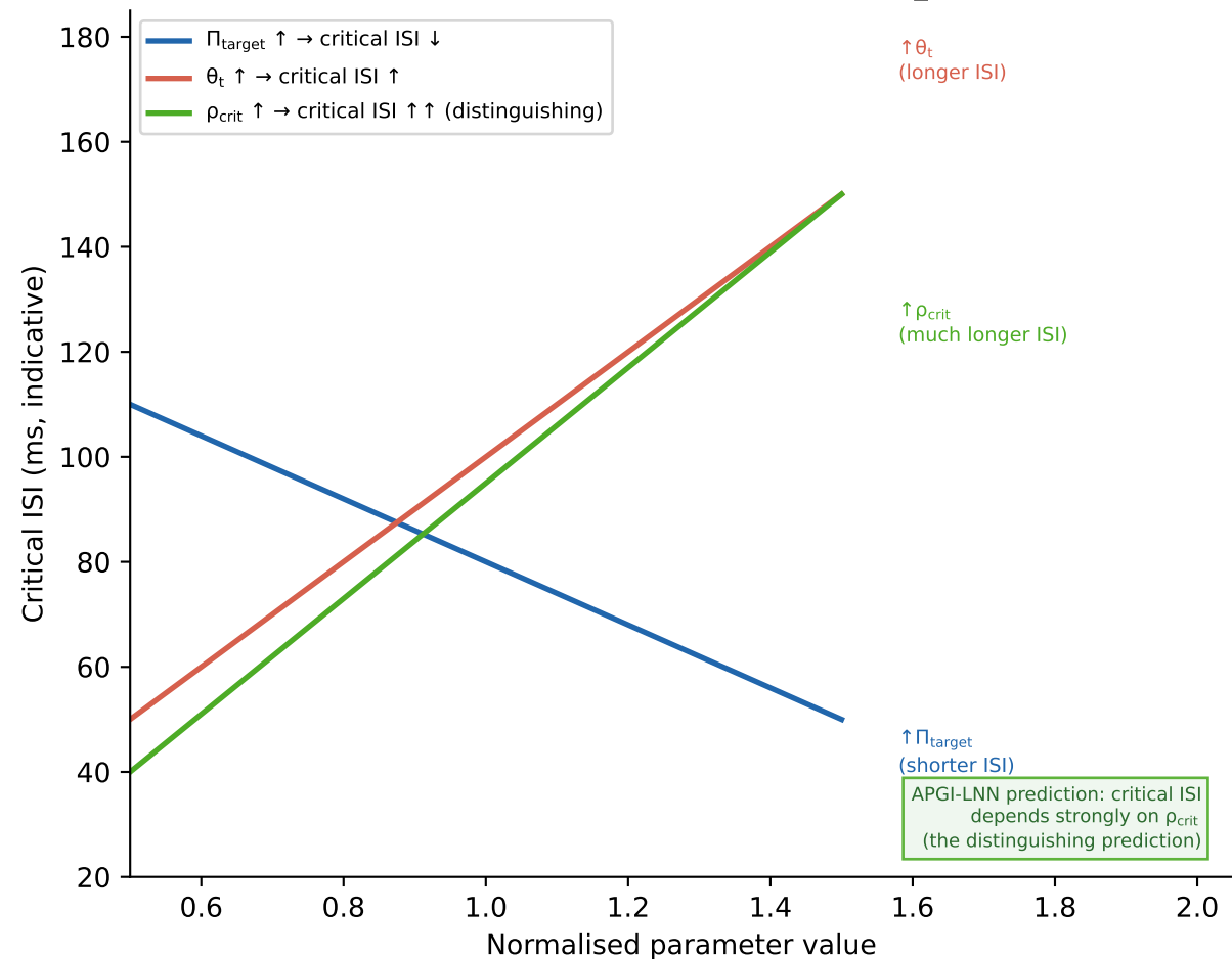
Critical ISI vs. normalised parameter value (distinguishing prediction: masking \propto \rho_{\text{crit}} )
