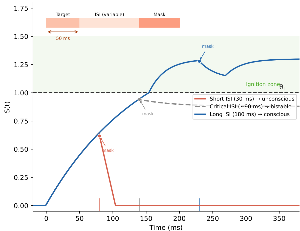
S(t) trajectories by ISI condition
