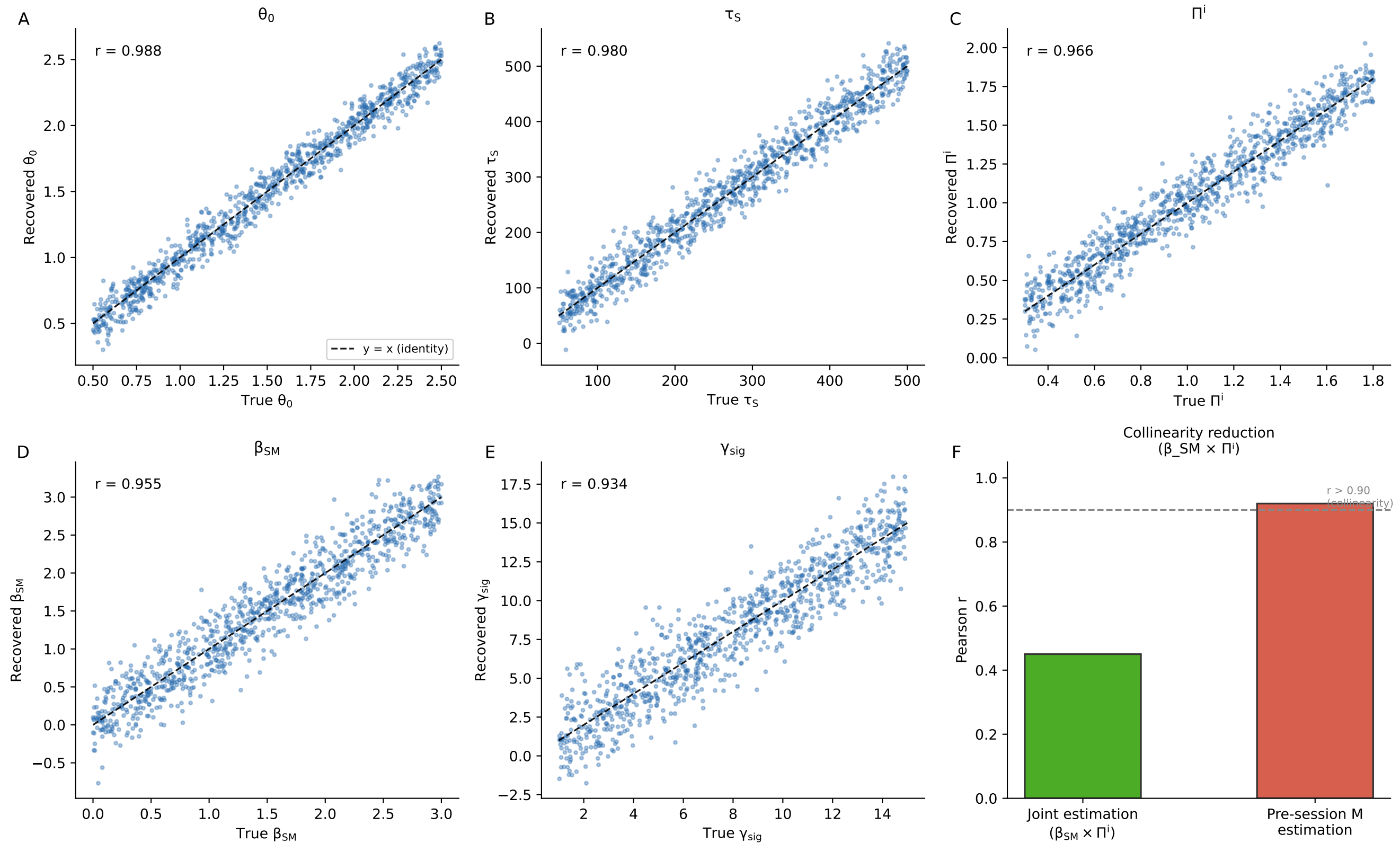
Figure S1 — Parameter Recovery Scatter Plots (N = 1,000 simulation runs) Appendix A.4, following Table S2
