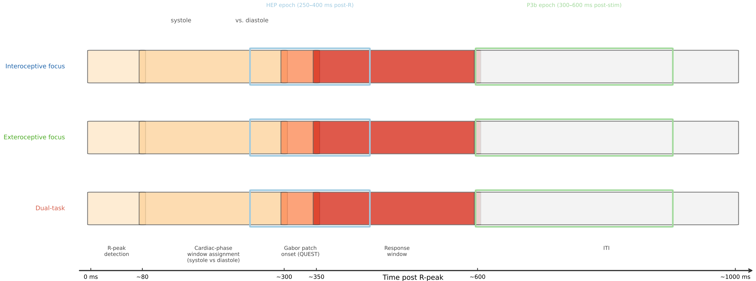
Figure S3 — Protocol 1 Trial-Timeline Schematic (Cardiac-Phase EEG) Appendix D.1, before Table S4
