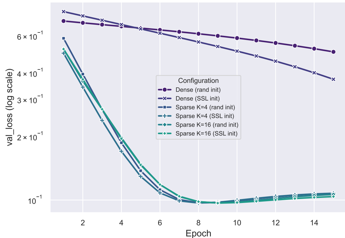
KNN TRA Parity — Dense vs Sparse Convergence (L=4, N=512)
